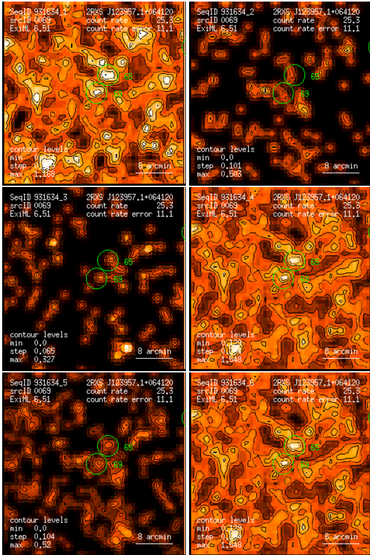
Figure 69: RASS 931634: detection 0069: band rate images, Gaussian filter: (1) PSPC channels 11 – 41, (2) 52 – 90, (3) 91 – 201, (4) 11 – 235, (5) 52 – 201, (6) 11 – 201. Broad band rates in counts/ks. Band rate contour levels in counts/ks/arcmin 2 .
