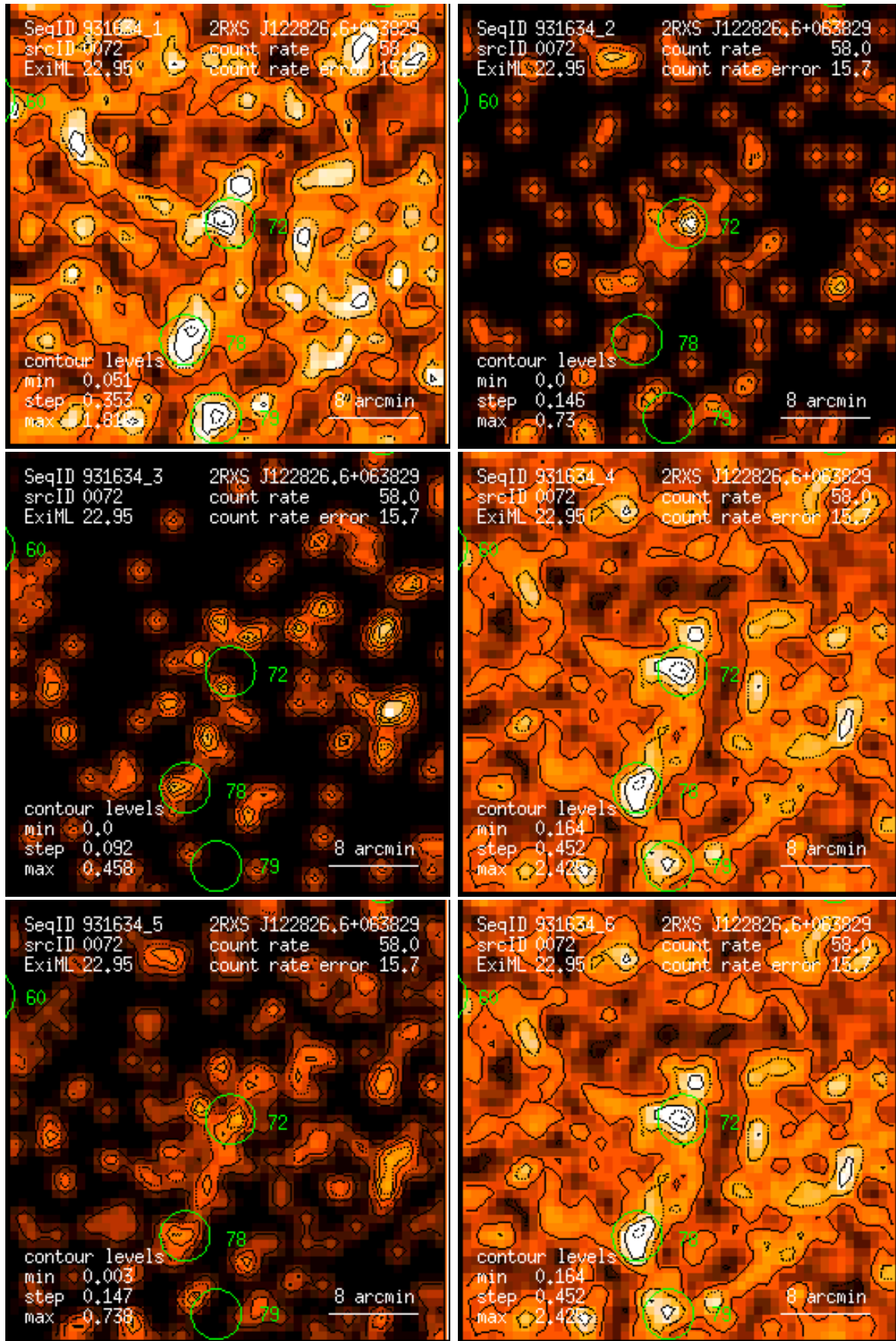
Figure 72: RASS 931634: detection 0072: band rate images, Gaussian filter: (1) PSPC channels 11 – 41, (2) 52 – 90, (3) 91 – 201, (4) 11 – 235, (5) 52 – 201, (6) 11 – 201. Broad band rates in counts/ks. Band rate contour levels in counts/ks/arcmin 2 .
