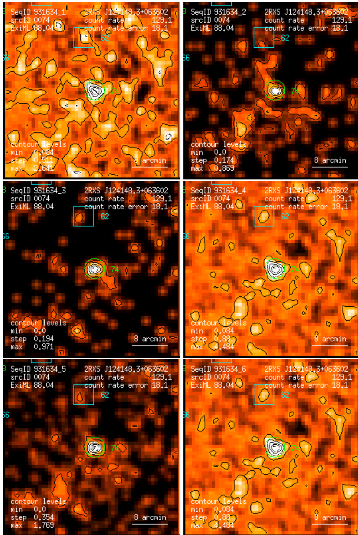
Figure 74: RASS 931634: detection 0074: band rate images, Gaussian filter: (1) PSPC channels 11 – 41, (2) 52 – 90, (3) 91 – 201, (4) 11 – 235, (5) 52 – 201, (6) 11 – 201. Broad band rates in counts/ks. Band rate contour levels in counts/ks/arcmin 2 .
