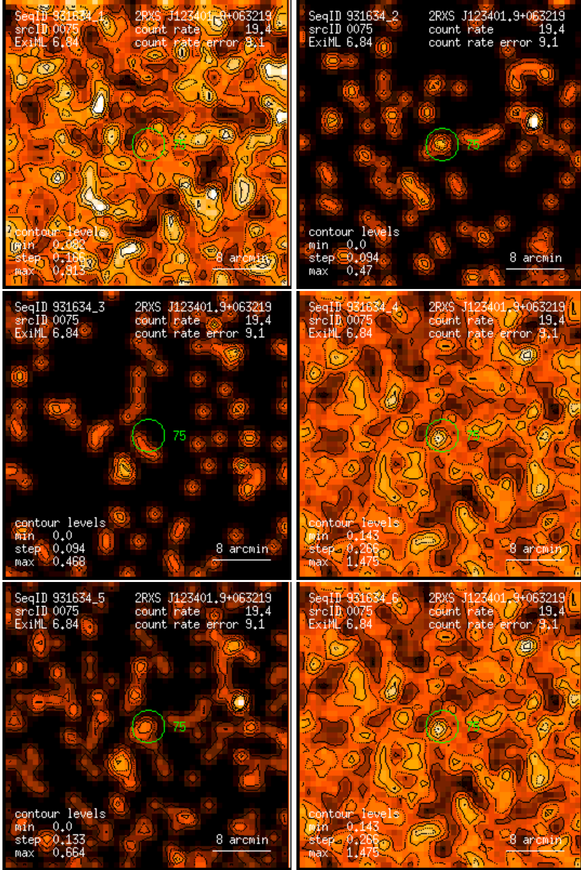
Figure 75: RASS 931634: detection 0075: band rate images, Gaussian filter: (1) PSPC channels 11 – 41, (2) 52 – 90, (3) 91 – 201, (4) 11 – 235, (5) 52 – 201, (6) 11 – 201. Broad band rates in counts/ks. Band rate contour levels in counts/ks/arcmin 2 .
