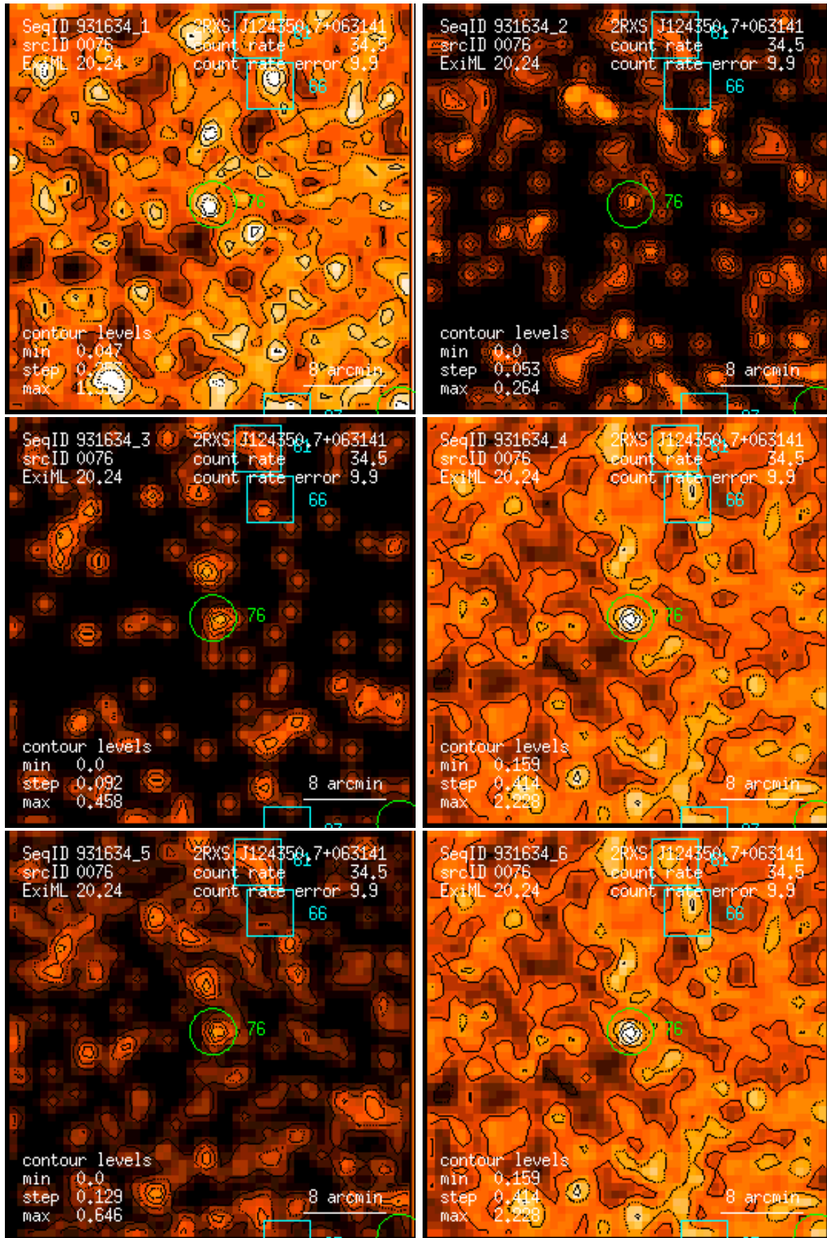
Figure 76: RASS 931634: detection 0076: band rate images, Gaussian filter: (1) PSPC channels 11 – 41, (2) 52 – 90, (3) 91 – 201, (4) 11 – 235, (5) 52 – 201, (6) 11 – 201. Broad band rates in counts/ks. Band rate contour levels in counts/ks/arcmin 2 .
