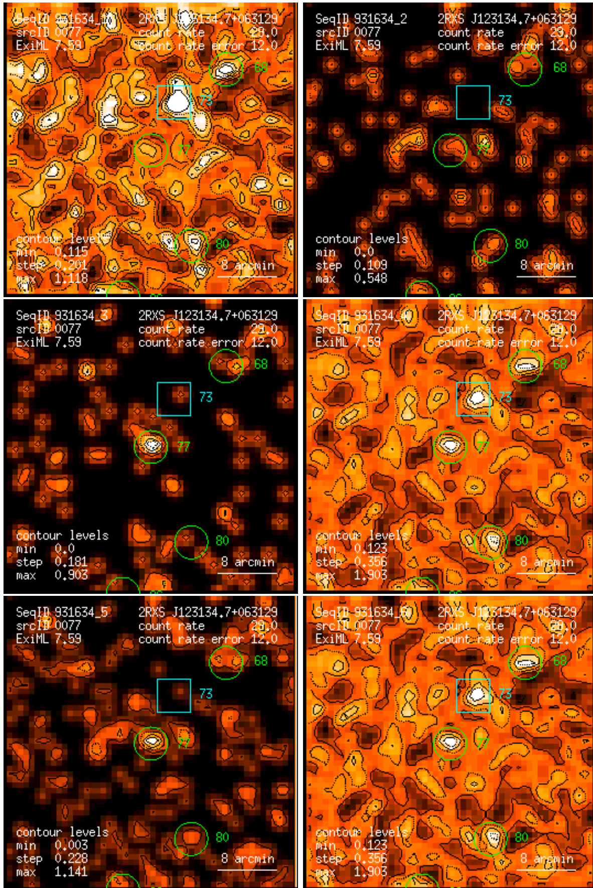
Figure 77: RASS 931634: detection 0077: band rate images, Gaussian filter: (1) PSPC channels 11 – 41, (2) 52 – 90, (3) 91 – 201, (4) 11 – 235, (5) 52 – 201, (6) 11 – 201. Broad band rates in counts/ks. Band rate contour levels in counts/ks/arcmin 2 .
