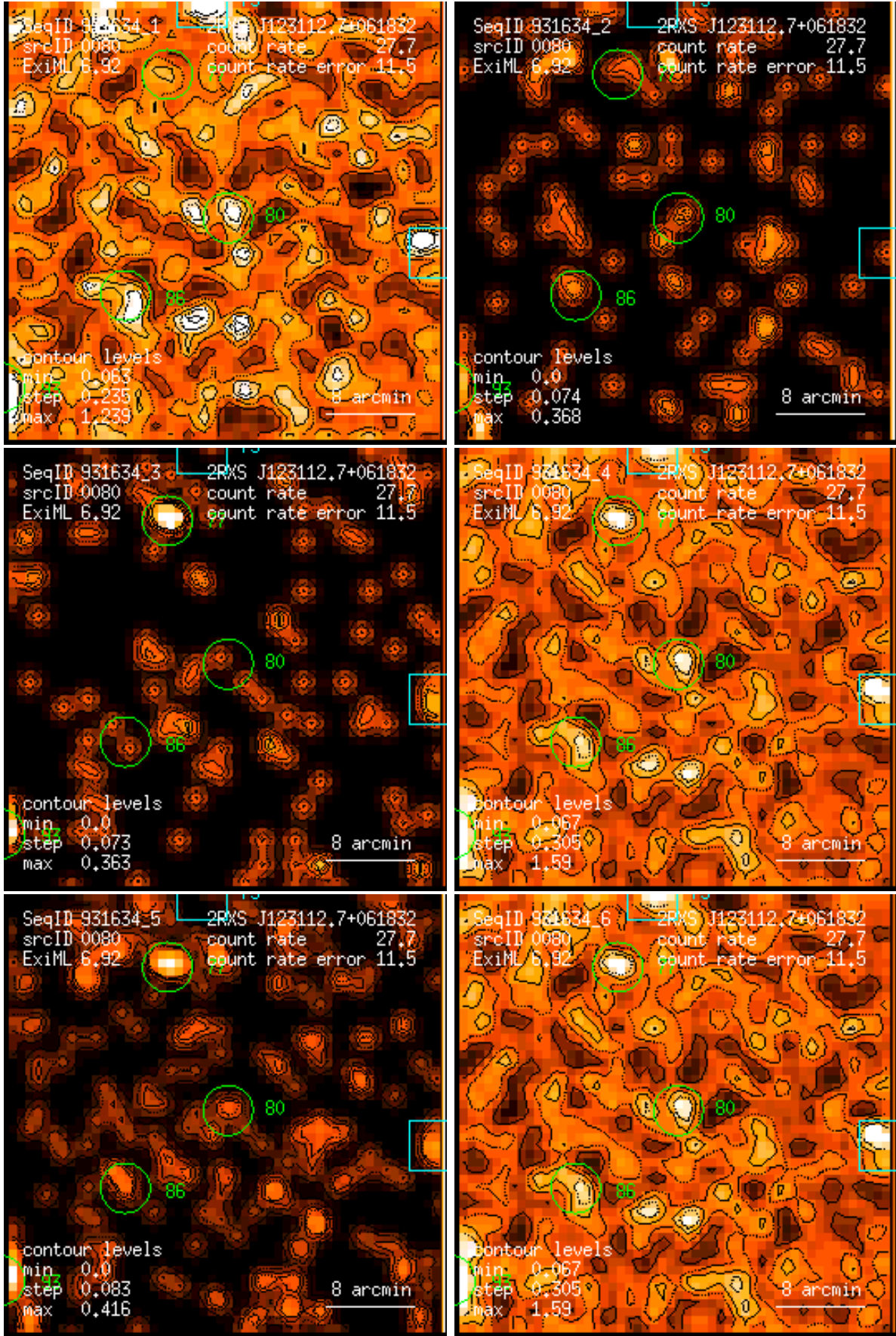
Figure 80: RASS 931634: detection 0080: band rate images, Gaussian filter: (1) PSPC channels 11 – 41, (2) 52 – 90, (3) 91 – 201, (4) 11 – 235, (5) 52 – 201, (6) 11 – 201. Broad band rates in counts/ks. Band rate contour levels in counts/ks/arcmin 2 .
