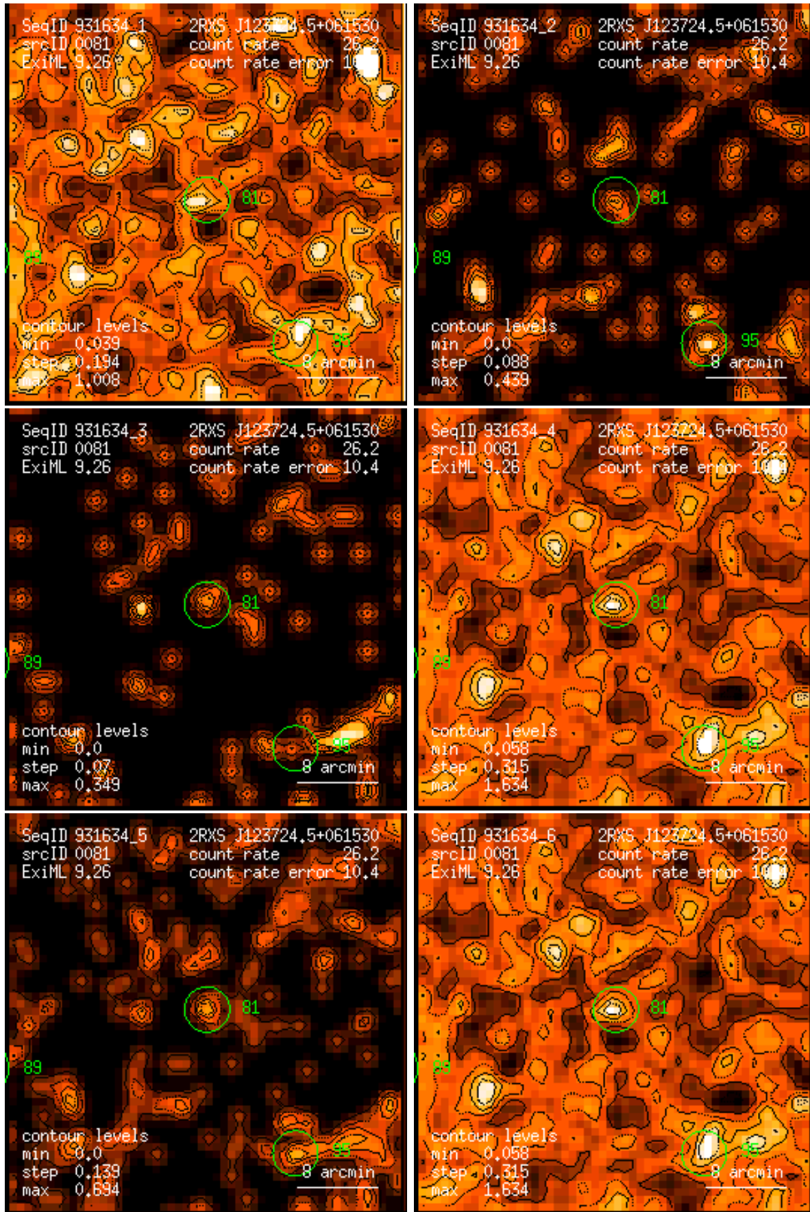
Figure 81: RASS 931634: detection 0081: band rate images, Gaussian filter: (1) PSPC channels 11 – 41, (2) 52 – 90, (3) 91 – 201, (4) 11 – 235, (5) 52 – 201, (6) 11 – 201. Broad band rates in counts/ks. Band rate contour levels in counts/ks/arcmin 2 .
