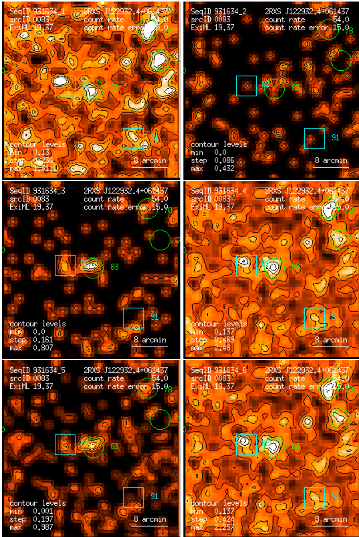
Figure 83: RASS 931634: detection 0083: band rate images, Gaussian filter: (1) PSPC channels 11 – 41, (2) 52 – 90, (3) 91 – 201, (4) 11 – 235, (5) 52 – 201, (6) 11 – 201. Broad band rates in counts/ks. Band rate contour levels in counts/ks/arcmin 2 .
