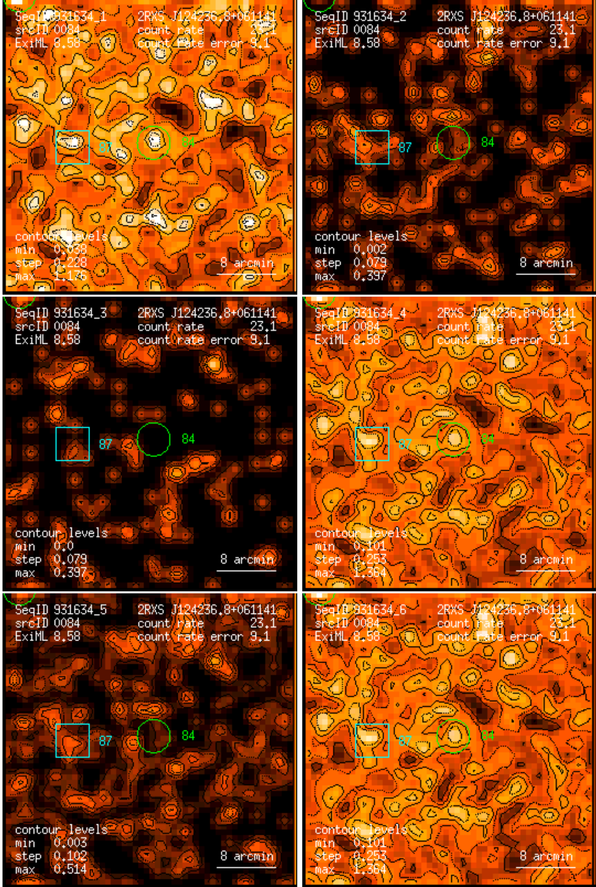
Figure 84: RASS 931634: detection 0084: band rate images, Gaussian filter: (1) PSPC channels 11 – 41, (2) 52 – 90, (3) 91 – 201, (4) 11 – 235, (5) 52 – 201, (6) 11 – 201. Broad band rates in counts/ks. Band rate contour levels in counts/ks/arcmin 2 .
