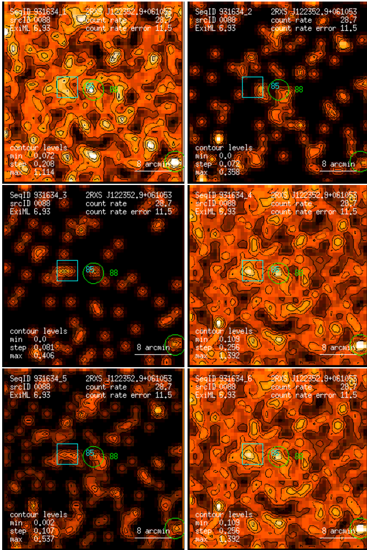
Figure 88: RASS 931634: detection 0088: band rate images, Gaussian filter: (1) PSPC channels 11 – 41, (2) 52 – 90, (3) 91 – 201, (4) 11 – 235, (5) 52 – 201, (6) 11 – 201. Broad band rates in counts/ks. Band rate contour levels in counts/ks/arcmin 2 .
