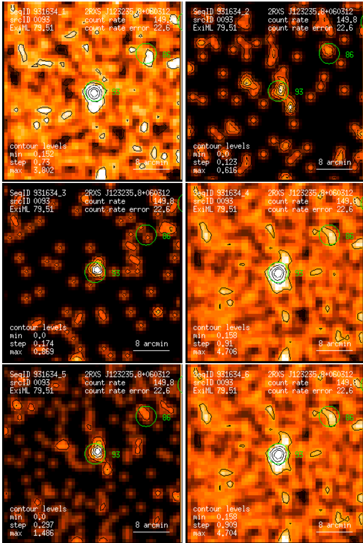
Figure 93: RASS 931634: detection 0093: band rate images, Gaussian filter: (1) PSPC channels 11 – 41, (2) 52 – 90, (3) 91 – 201, (4) 11 – 235, (5) 52 – 201, (6) 11 – 201. Broad band rates in counts/ks. Band rate contour levels in counts/ks/arcmin 2 .
