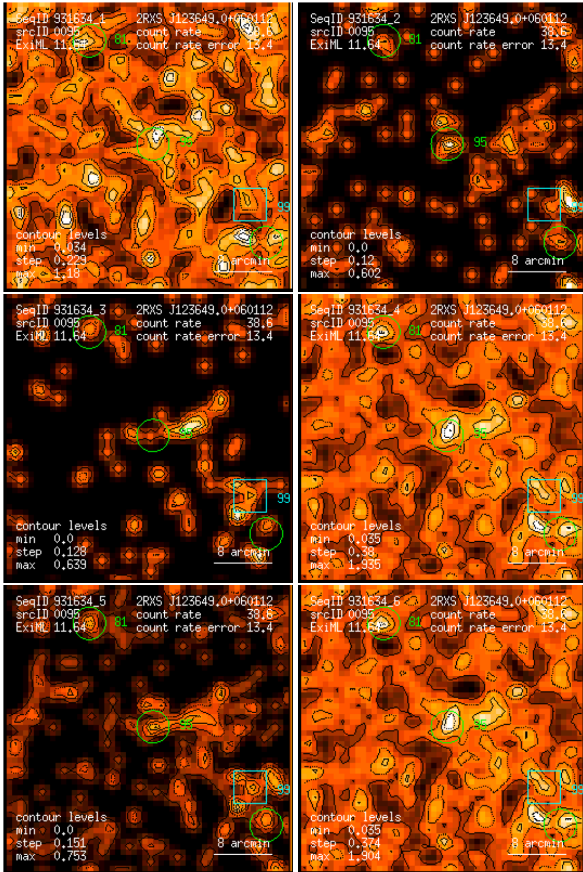
Figure 95: RASS 931634: detection 0095: band rate images, Gaussian filter: (1) PSPC channels 11 – 41, (2) 52 – 90, (3) 91 – 201, (4) 11 – 235, (5) 52 – 201, (6) 11 – 201. Broad band rates in counts/ks. Band rate contour levels in counts/ks/arcmin 2 .
