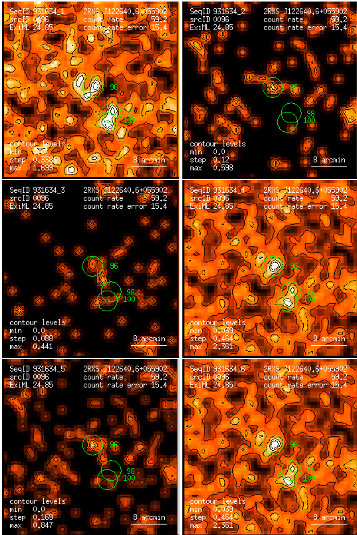
Figure 96: RASS 931634: detection 0096: band rate images, Gaussian filter: (1) PSPC channels 11 – 41, (2) 52 – 90, (3) 91 – 201, (4) 11 – 235, (5) 52 – 201, (6) 11 – 201. Broad band rates in counts/ks. Band rate contour levels in counts/ks/arcmin 2 .
