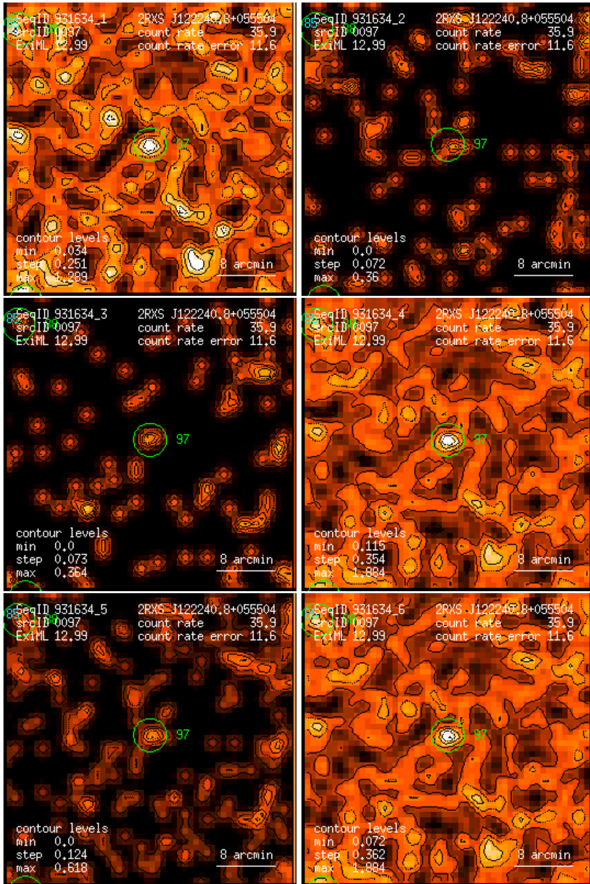
Figure 97: RASS 931634: detection 0097: band rate images, Gaussian filter: (1) PSPC channels 11 – 41, (2) 52 – 90, (3) 91 – 201, (4) 11 – 235, (5) 52 – 201, (6) 11 – 201. Broad band rates in counts/ks. Band rate contour levels in counts/ks/arcmin 2 .
