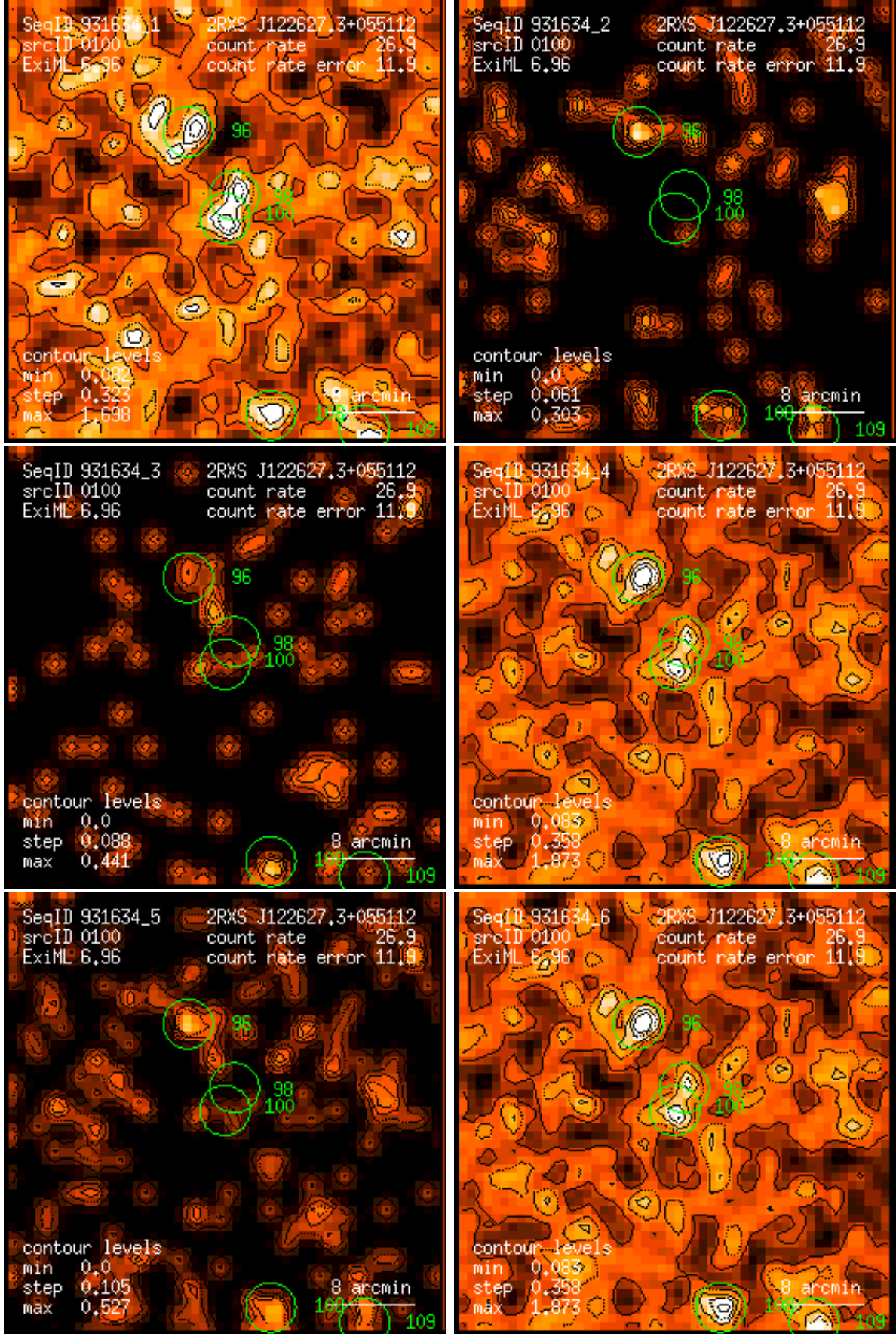
Figure 100: RASS 931634: detection 0100: band rate images, Gaussian filter: (1) PSPC channels 11 – 41, (2) 52 – 90, (3) 91 – 201, (4) 11 – 235, (5) 52 – 201, (6) 11 – 201. Broad band rates in counts/ks. Band rate contour levels in counts/ks/arcmin 2 .
