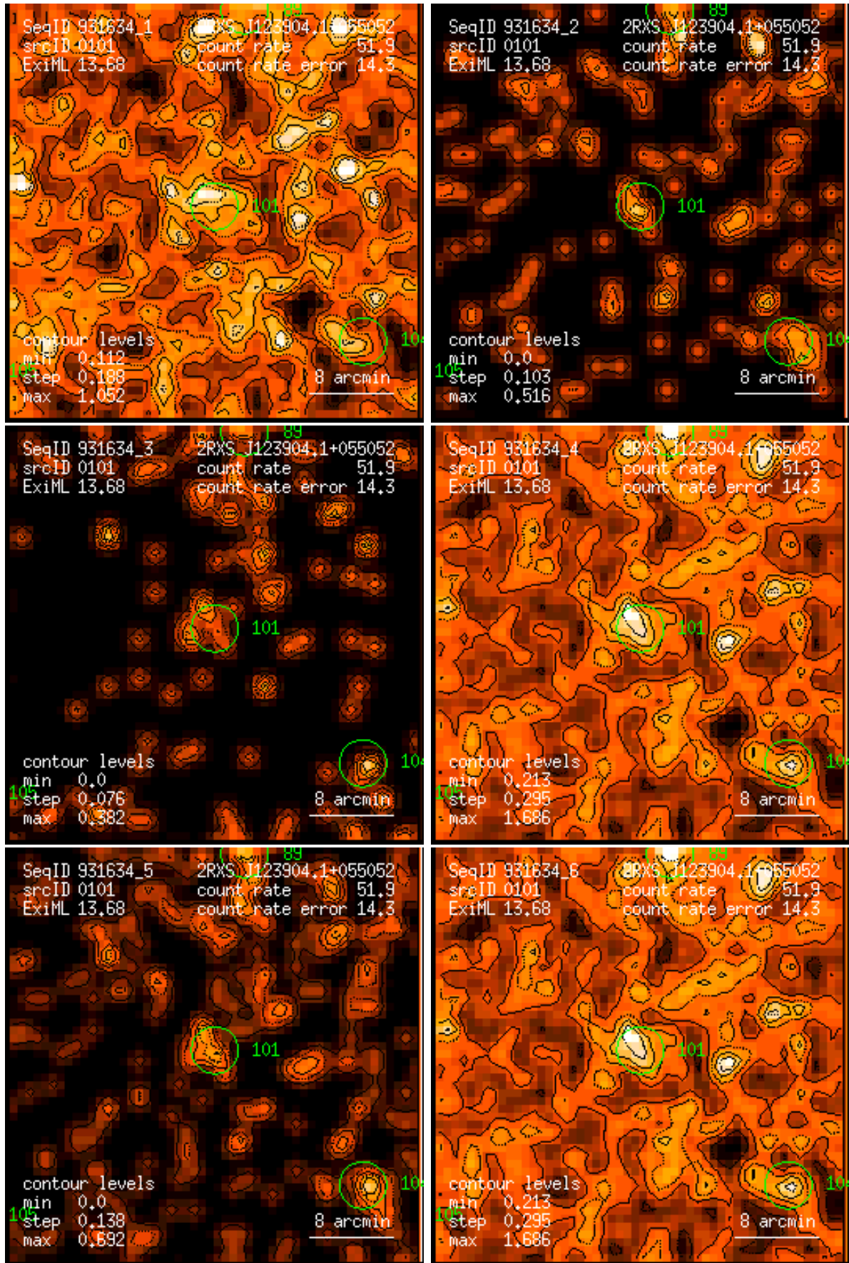
Figure 101: RASS 931634: detection 0101: band rate images, Gaussian filter: (1) PSPC channels 11 – 41, (2) 52 – 90, (3) 91 – 201, (4) 11 – 235, (5) 52 – 201, (6) 11 – 201. Broad band rates in counts/ks. Band rate contour levels in counts/ks/arcmin 2 .
