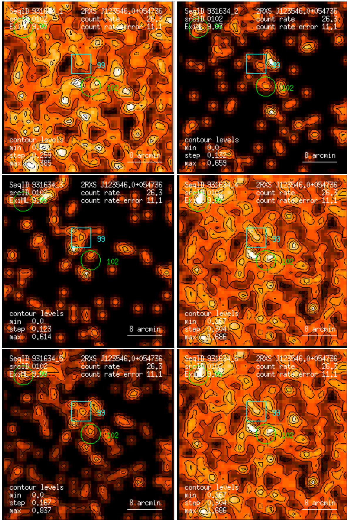
Figure 102: RASS 931634: detection 0102: band rate images, Gaussian filter: (1) PSPC channels 11 – 41, (2) 52 – 90, (3) 91 – 201, (4) 11 – 235, (5) 52 – 201, (6) 11 – 201. Broad band rates in counts/ks. Band rate contour levels in counts/ks/arcmin 2 .
