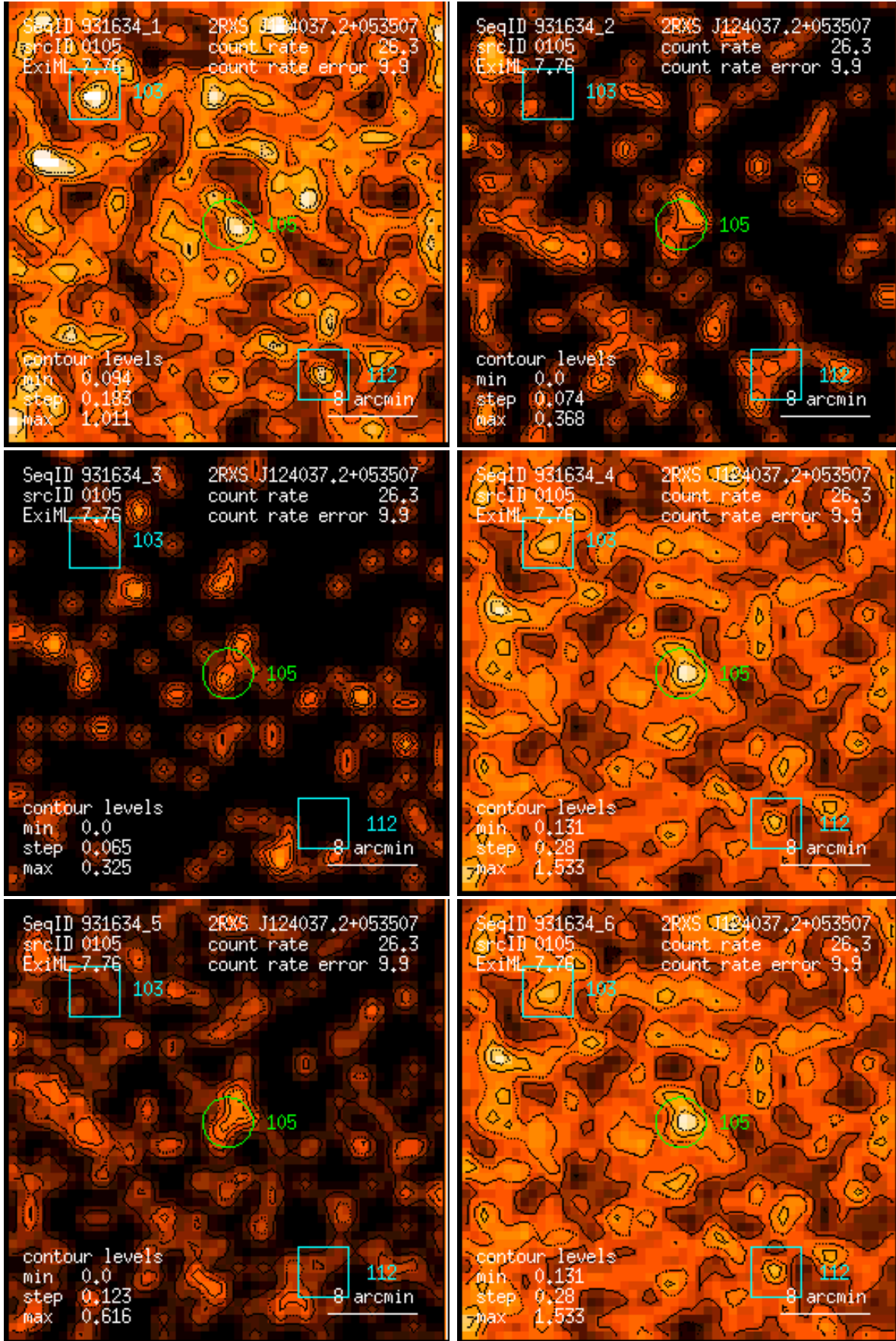
Figure 105: RASS 931634: detection 0105: band rate images, Gaussian filter: (1) PSPC channels 11 – 41, (2) 52 – 90, (3) 91 – 201, (4) 11 – 235, (5) 52 – 201, (6) 11 – 201. Broad band rates in counts/ks. Band rate contour levels in counts/ks/arcmin 2 .
