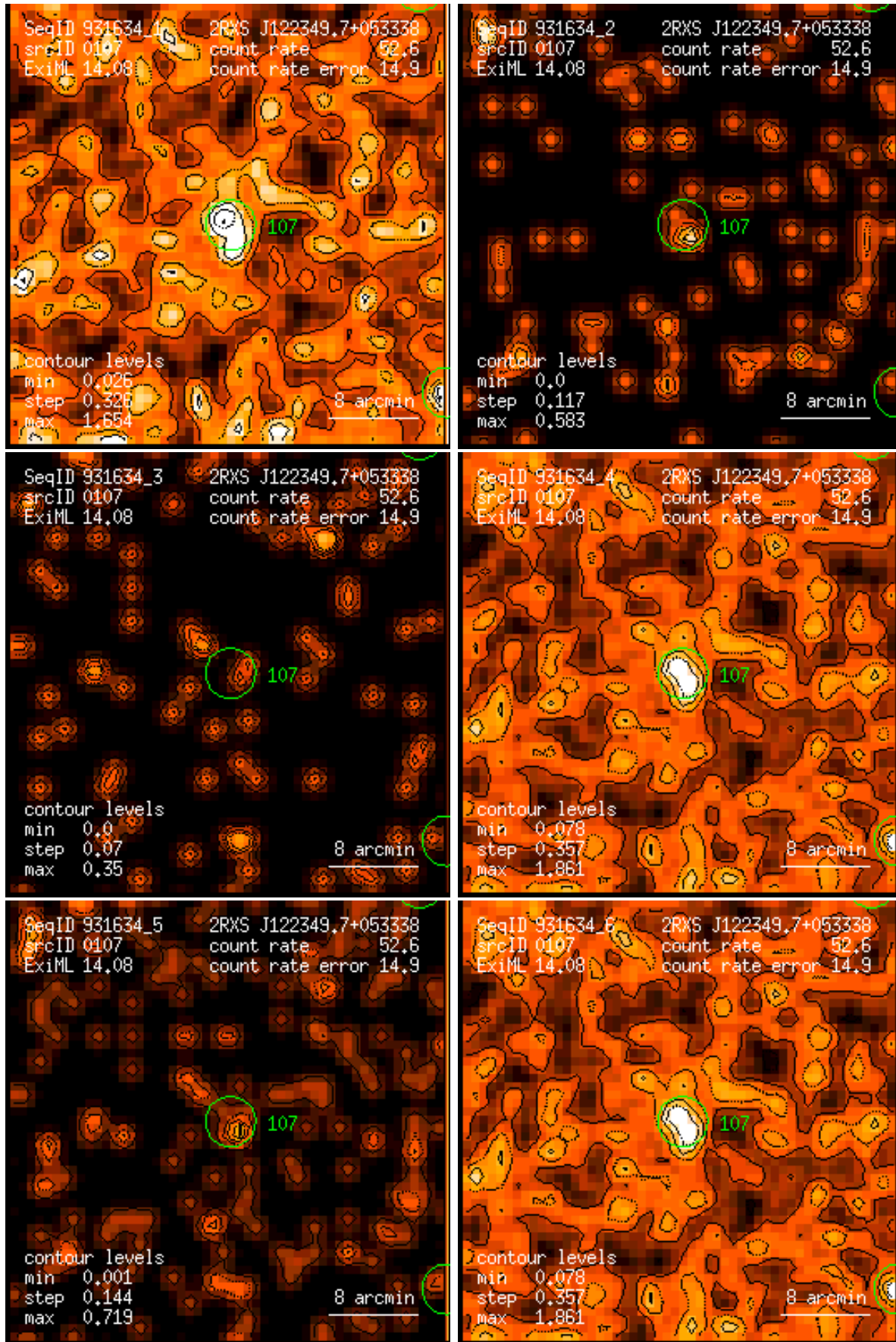
Figure 107: RASS 931634: detection 0107: band rate images, Gaussian filter: (1) PSPC channels 11 – 41, (2) 52 – 90, (3) 91 – 201, (4) 11 – 235, (5) 52 – 201, (6) 11 – 201. Broad band rates in counts/ks. Band rate contour levels in counts/ks/arcmin 2 .
