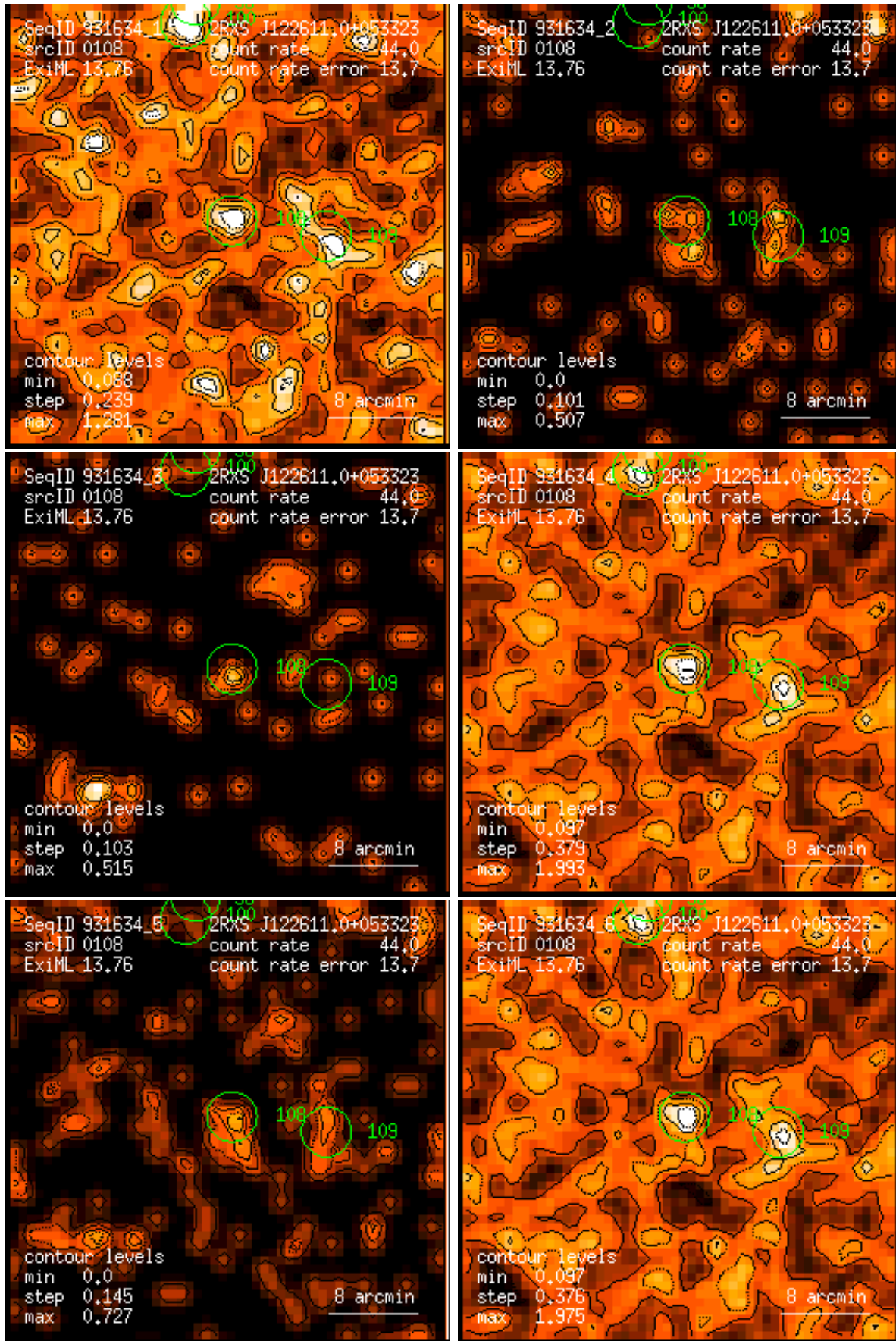
Figure 108: RASS 931634: detection 0108: band rate images, Gaussian filter: (1) PSPPC channels 11 – 41, (2) 52 – 90, (3) 91 – 201, (4) 11 – 235, (5) 52 – 201, (6) 11 – 201. Broad band rates in counts/ks. Band rate contour levels in counts/ks/arcmin 2 .
