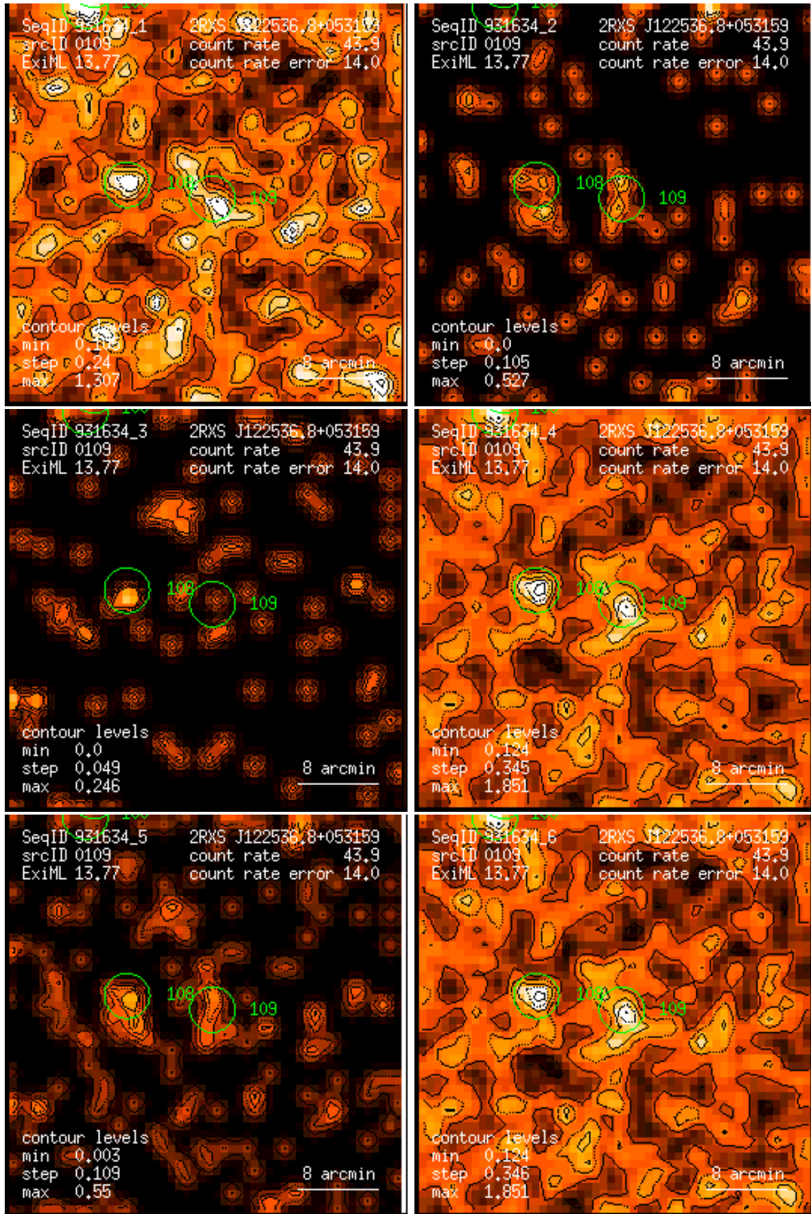
Figure 109: RASS 931634: detection 0109: band rate images, Gaussian filter: (1) PSPC channels 11 – 41, (2) 52 – 90, (3) 91 – 201, (4) 11 – 235, (5) 52 – 201, (6) 11 – 201. Broad band rates in counts/ks. Band rate contour levels in counts/ks/arcmin 2 .
