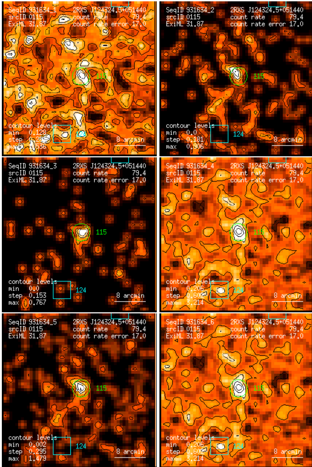
Figure 115: RASS 931634: detection 0115: band rate images, Gaussian filter: (1) PSPC channels 11 – 41, (2) 52 – 90, (3) 91 – 201, (4) 11 – 235, (5) 52 – 201, (6) 11 – 201. Broad band rates in counts/ks. Band rate contour levels in counts/ks/arcmin 2 .
