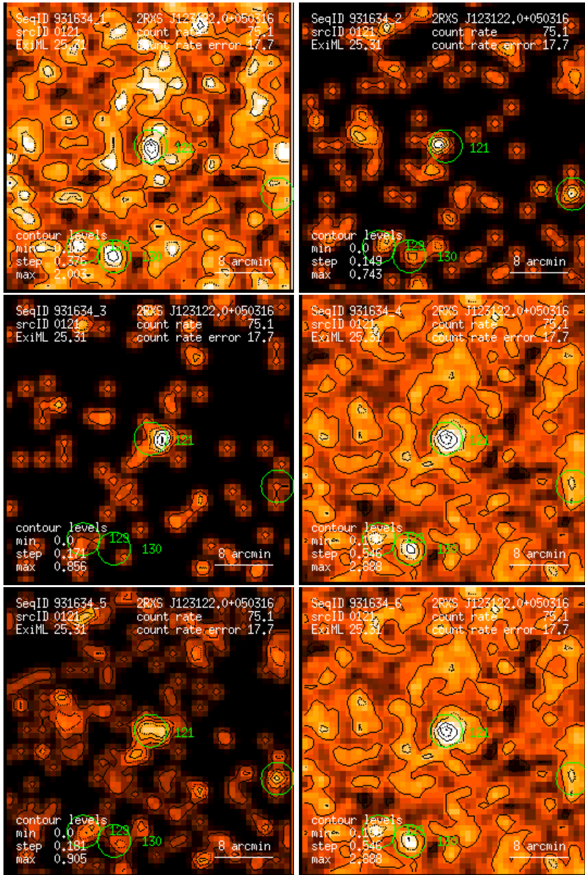
Figure 121: RASS 931634: detection 0121: band rate images, Gaussian filter: (1) PSPC channels 11 – 41, (2) 52 – 90, (3) 91 – 201, (4) 11 – 235, (5) 52 – 201, (6) 11 – 201. Broad band rates in counts/ks. Band rate contour levels in counts/ks/arcmin 2 .
