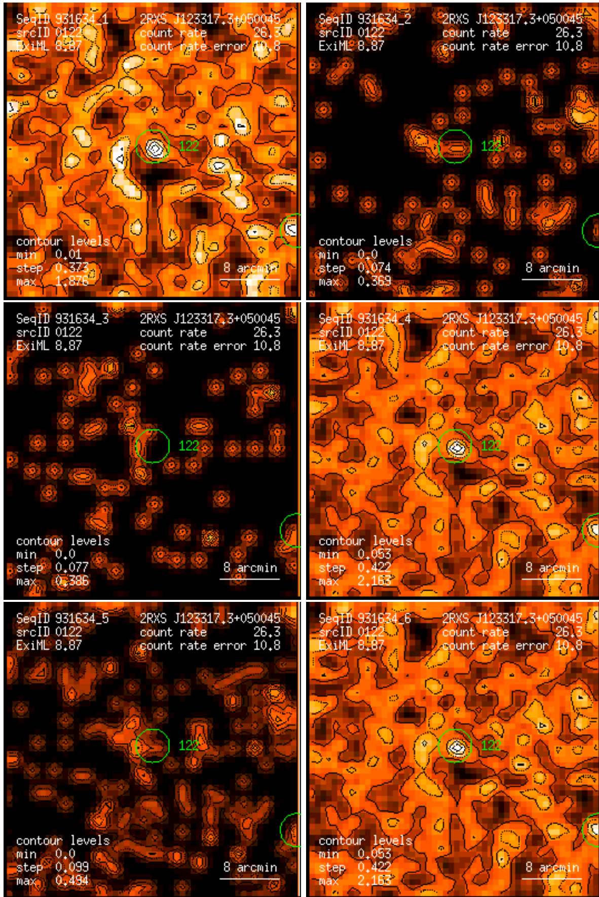
Figure 122: RASS 931634: detection 0122: band rate images, Gaussian filter: (1) PSPC channels 11 – 41, (2) 52 – 90, (3) 91 – 201, (4) 11 – 235, (5) 52 – 201, (6) 11 – 201. Broad band rates in counts/ks. Band rate contour levels in counts/ks/arcmin 2 .
