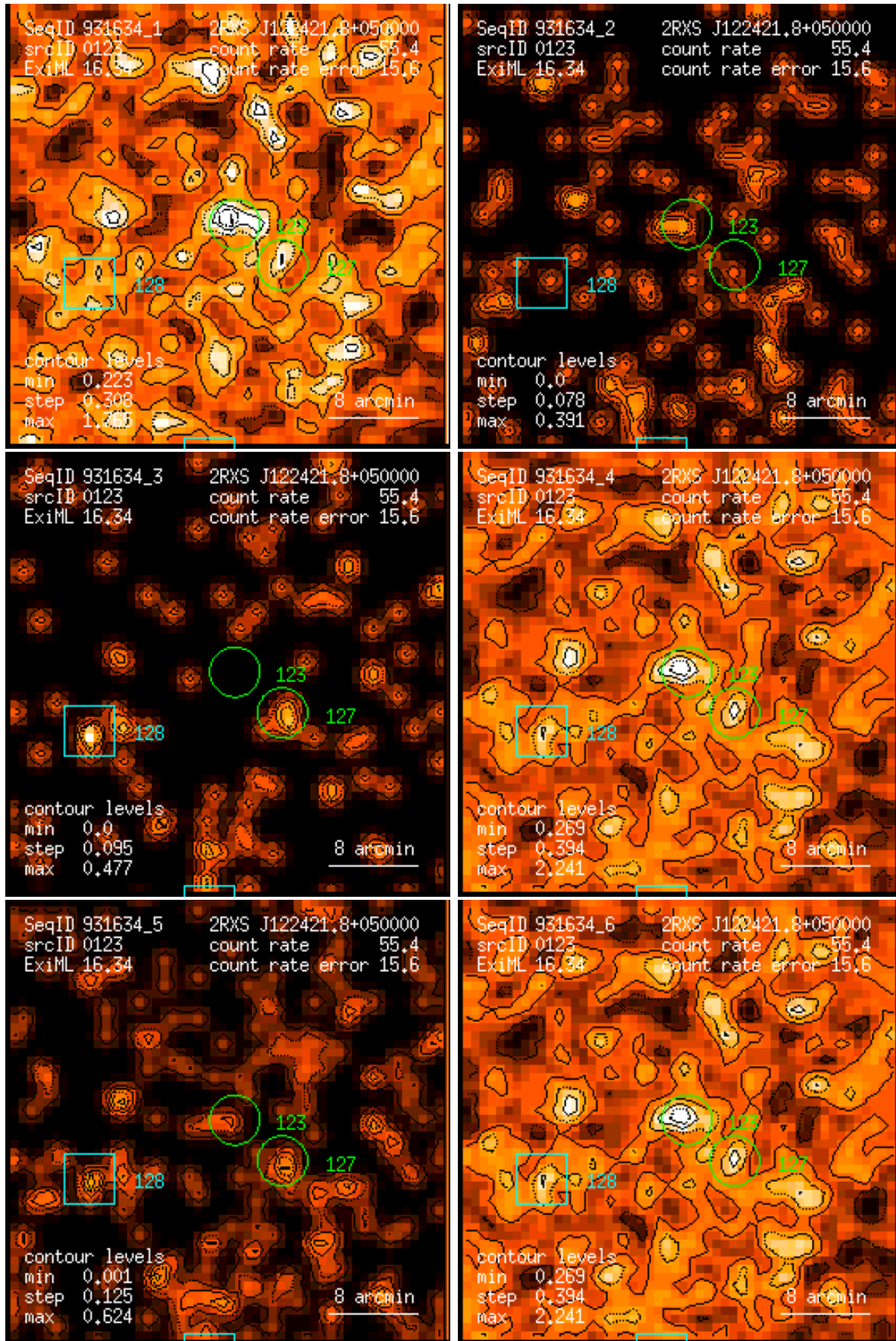
Figure 123: RASS 931634: detection 0123: band rate images, Gaussian filter: (1) PSPC channels 11 – 41, (2) 52 – 90, (3) 91 – 201, (4) 11 – 235, (5) 52 – 201, (6) 11 – 201. Broad band rates in counts/ks. Band rate contour levels in counts/ks/arcmin 2 .
