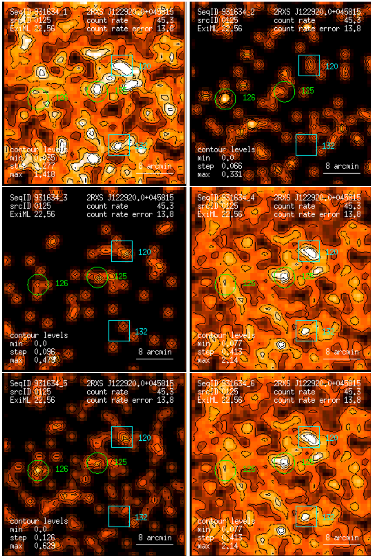
Figure 125: RASS 931634: detection 0125: band rate images, Gaussian filter: (1) PSPC channels 11 – 41, (2) 52 – 90, (3) 91 – 201, (4) 11 – 235, (5) 52 – 201, (6) 11 – 201. Broad band rates in counts/ks. Band rate contour levels in counts/ks/arcmin 2 .
