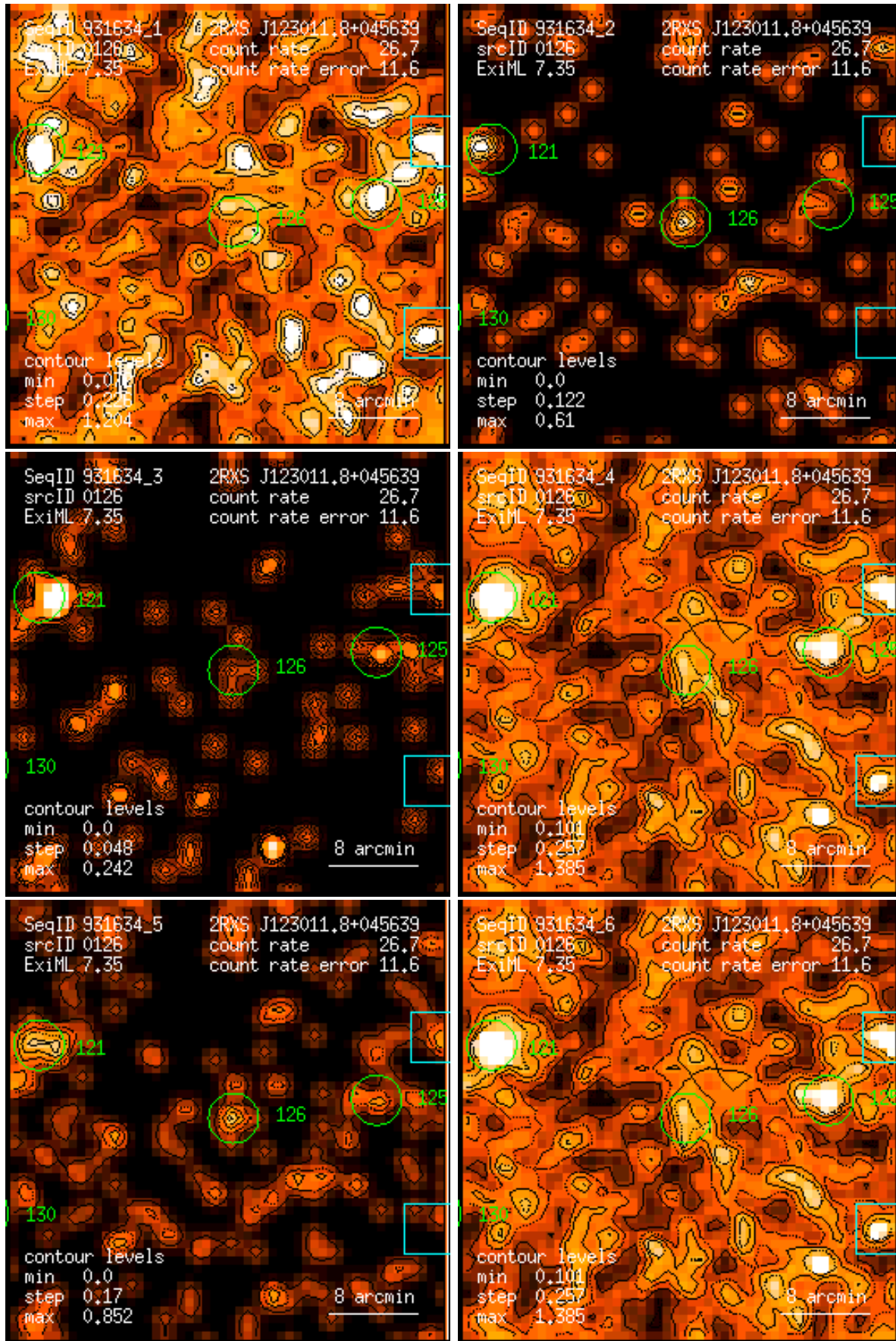
Figure 126: RASS 931634: detection 0126: band rate images, Gaussian filter: (1) PSPC channels 11 – 41, (2) 52 – 90, (3) 91 – 201, (4) 11 – 235, (5) 52 – 201, (6) 11 – 201. Broad band rates in counts/ks. Band rate contour levels in counts/ks/arcmin 2 .
