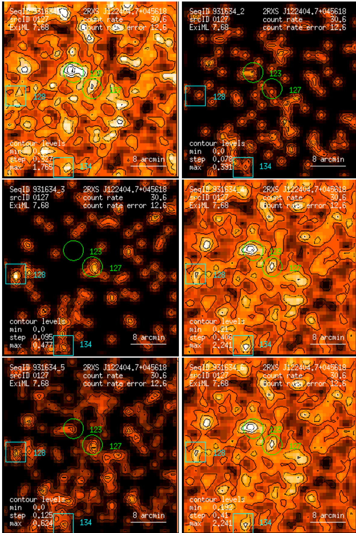
Figure 127: RASS 931634: detection 0127: band rate images, Gaussian filter: (1) PSPC channels 11 – 41, (2) 52 – 90, (3) 91 – 201, (4) 11 – 235, (5) 52 – 201, (6) 11 – 201. Broad band rates in counts/ks. Band rate contour levels in counts/ks/arcmin 2 .
