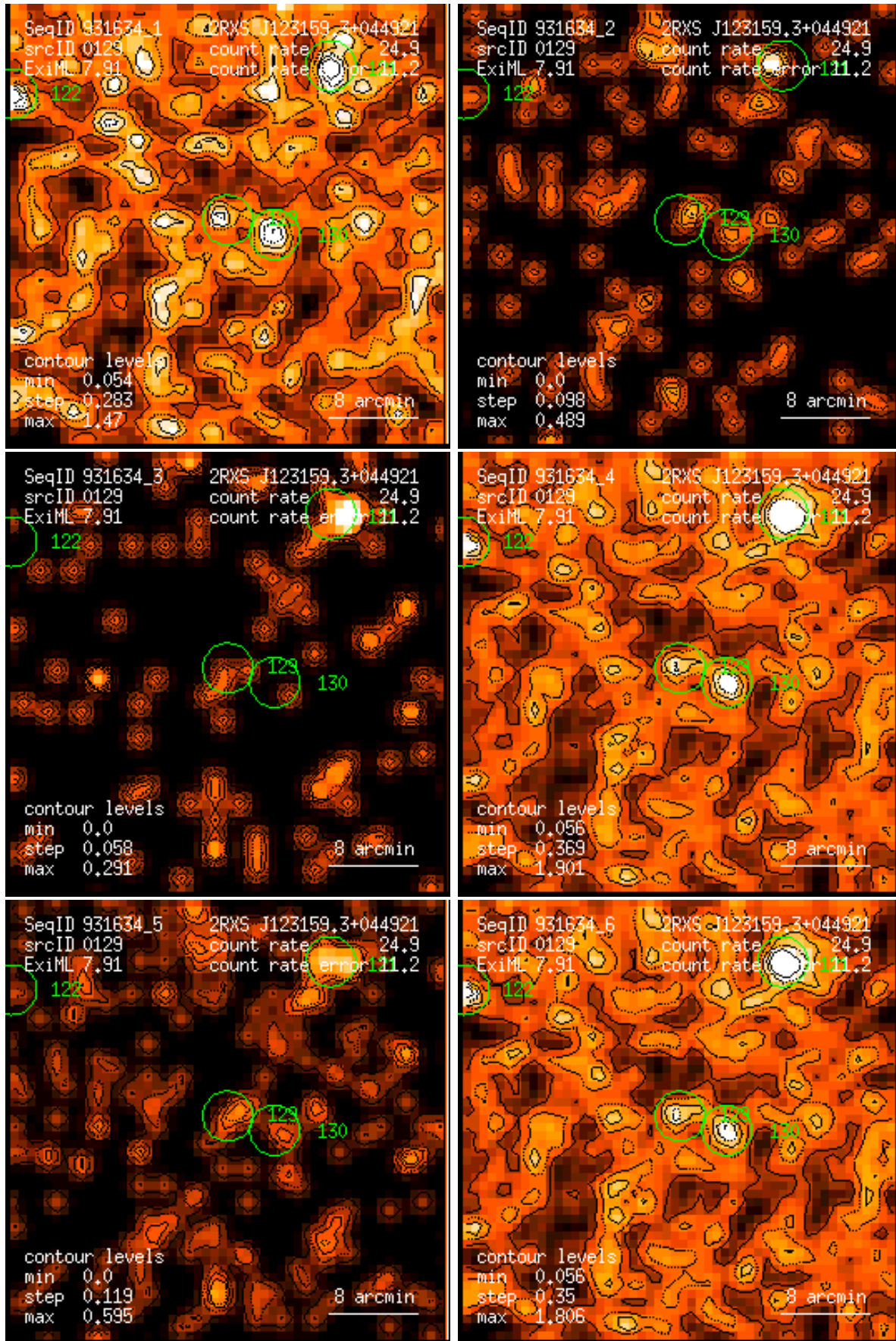
Figure 129: RASS 931634: detection 0129: band rate images, Gaussian filter: (1) PSPPC channels 11 – 41, (2) 52 – 90, (3) 91 – 201, (4) 11 – 235, (5) 52 – 201, (6) 11 – 201. Broad band rates in counts/ks. Band rate contour levels in counts/ks/arcmin 2 .
