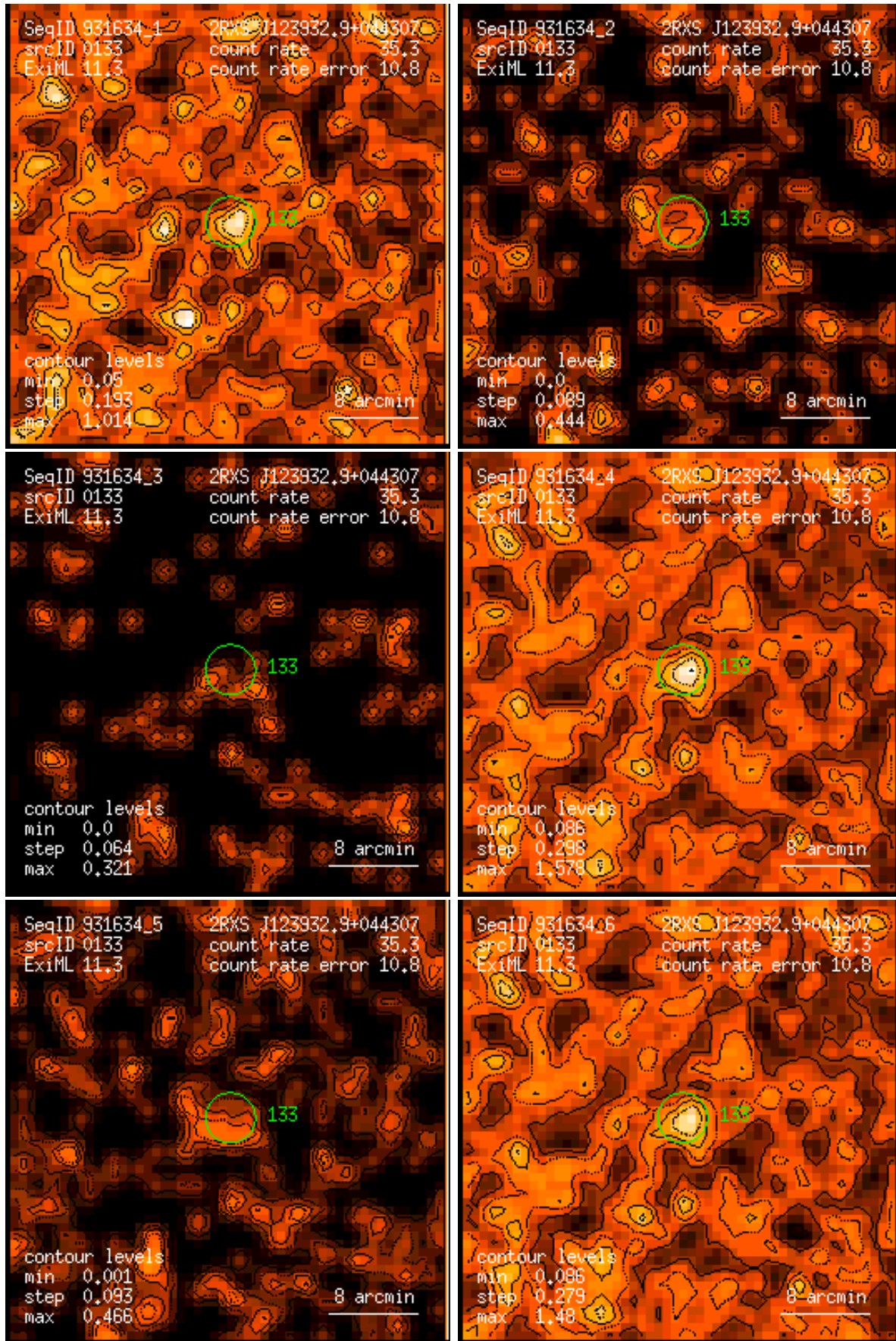
Figure 133: RASS 931634: detection 0133: band rate images, Gaussian filter: (1) PSPC channels 11 – 41, (2) 52 – 90, (3) 91 – 201, (4) 11 – 235, (5) 52 – 201, (6) 11 – 201. Broad band rates in counts/ks. Band rate contour levels in counts/ks/arcmin 2 .
