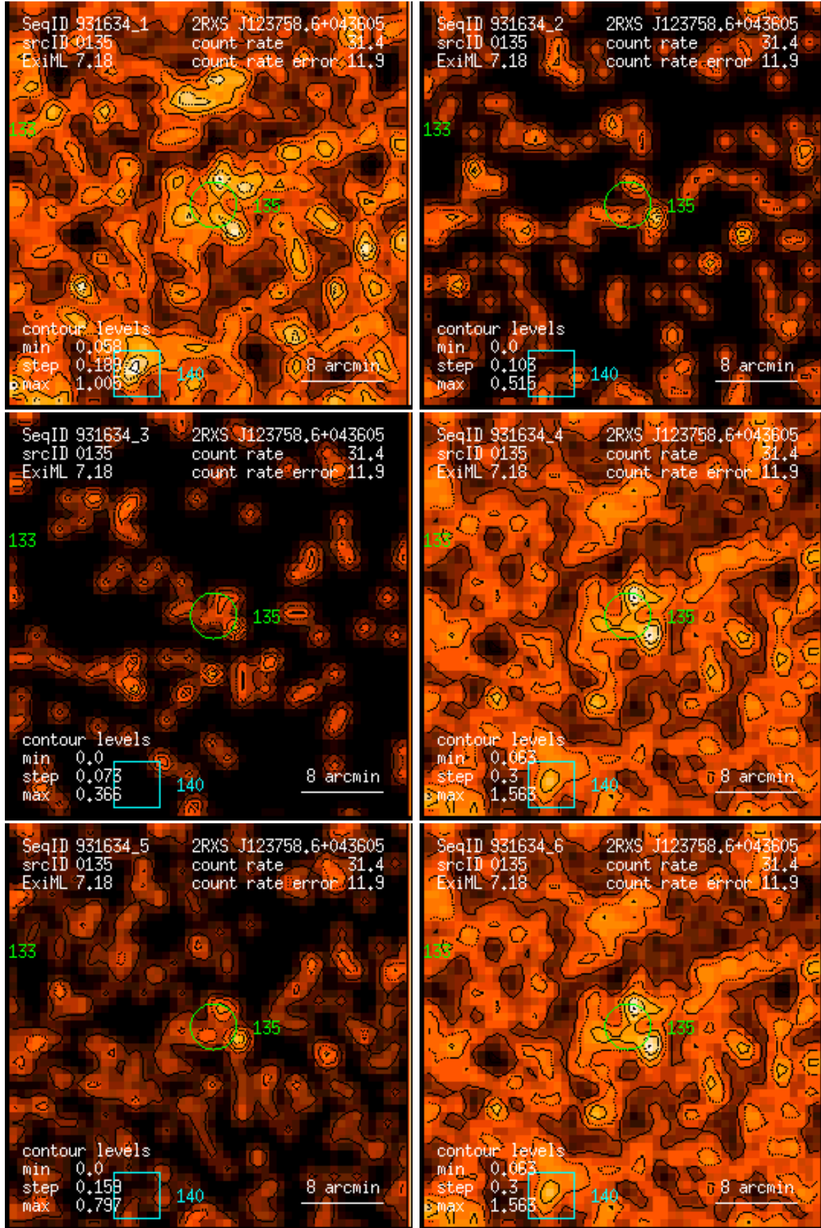
Figure 135: RASS 931634: detection 0135: band rate images, Gaussian filter: (1) PSPC channels 11 – 41, (2) 52 – 90, (3) 91 – 201, (4) 11 – 235, (5) 52 – 201, (6) 11 – 201. Broad band rates in counts/ks. Band rate contour levels in counts/ks/arcmin 2 .
