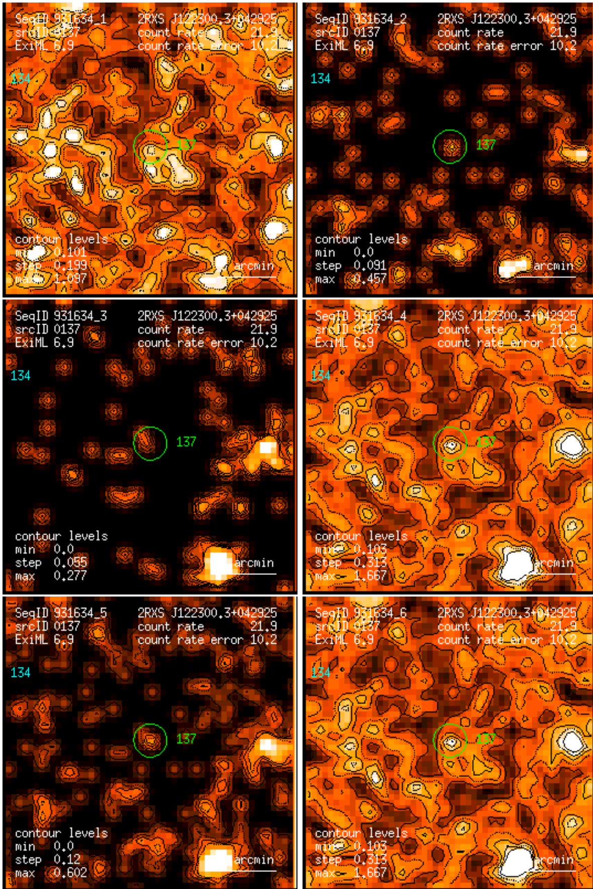
Figure 137: RASS 931634: detection 0137: band rate images, Gaussian filter: (1) PSPC channels 11 – 41, (2) 52 – 90, (3) 91 – 201, (4) 11 – 235, (5) 52 – 201, (6) 11 – 201. Broad band rates in counts/ks. Band rate contour levels in counts/ks/arcmin 2 .
