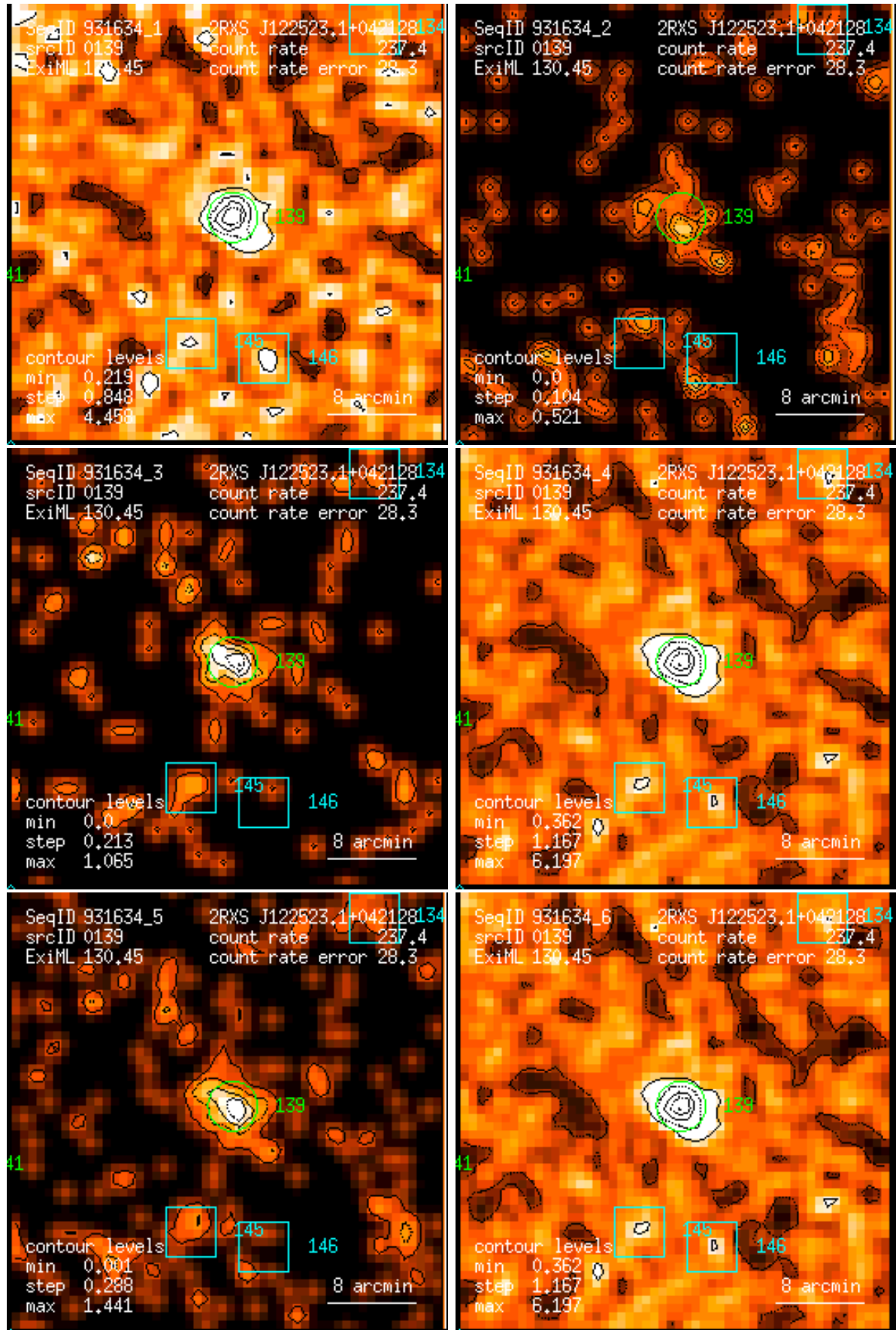
Figure 139: RASS 931634: detection 0139: band rate images, Gaussian filter: (1) PSPC channels 11 – 41, (2) 52 – 90, (3) 91 – 201, (4) 11 – 235, (5) 52 – 201, (6) 11 – 201. Broad band rates in counts/ks. Band rate contour levels in counts/ks/arcmin 2 .
