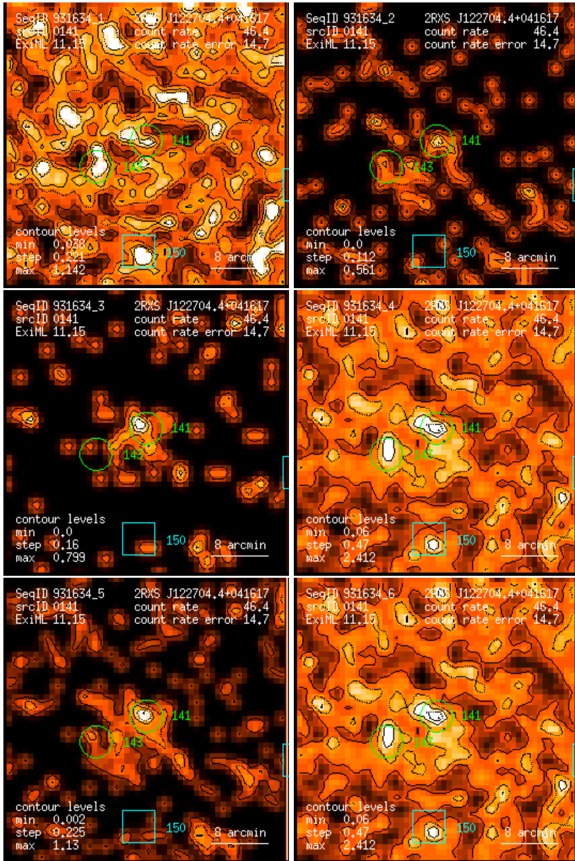
Figure 141: RASS 931634: detection 0141: band rate images, Gaussian filter: (1) PSPC channels 11 – 41, (2) 52 – 90, (3) 91 – 201, (4) 11 – 235, (5) 52 – 201, (6) 11 – 201. Broad band rates in counts/ks. Band rate contour levels in counts/ks/arcmin 2 .
