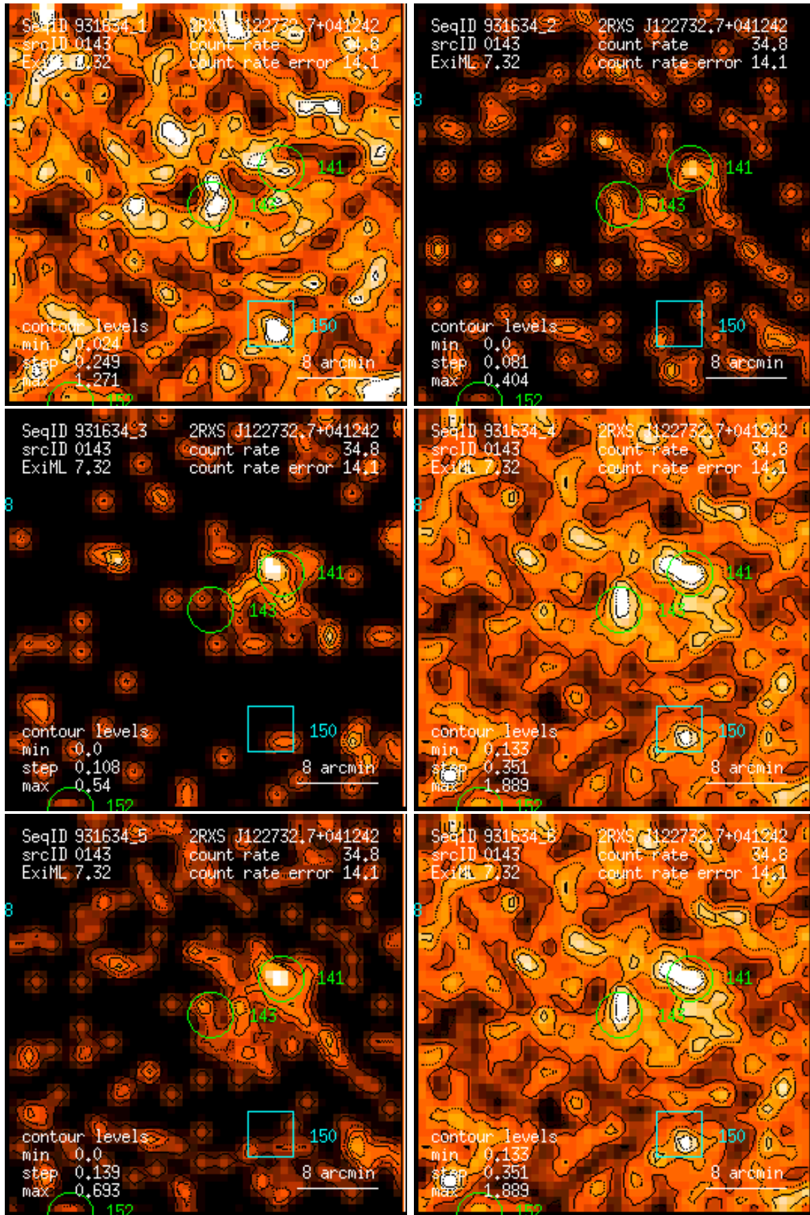
Figure 143: RASS 931634: detection 0143: band rate images, Gaussian filter: (1) PSPC channels 11 – 41, (2) 52 – 90, (3) 91 – 201, (4) 11 – 235, (5) 52 – 201, (6) 11 – 201. Broad band rates in counts/ks. Band rate contour levels in counts/ks/arcmin 2 .
