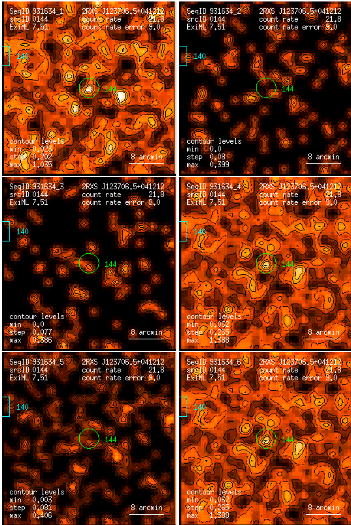
Figure 144: RASS 931634: detection 0144: band rate images, Gaussian filter: (1) PSPC channels 11 – 41, (2) 52 – 90, (3) 91 – 201, (4) 11 – 235, (5) 52 – 201, (6) 11 – 201. Broad band rates in counts/ks. Band rate contour levels in counts/ks/arcmin 2 .
