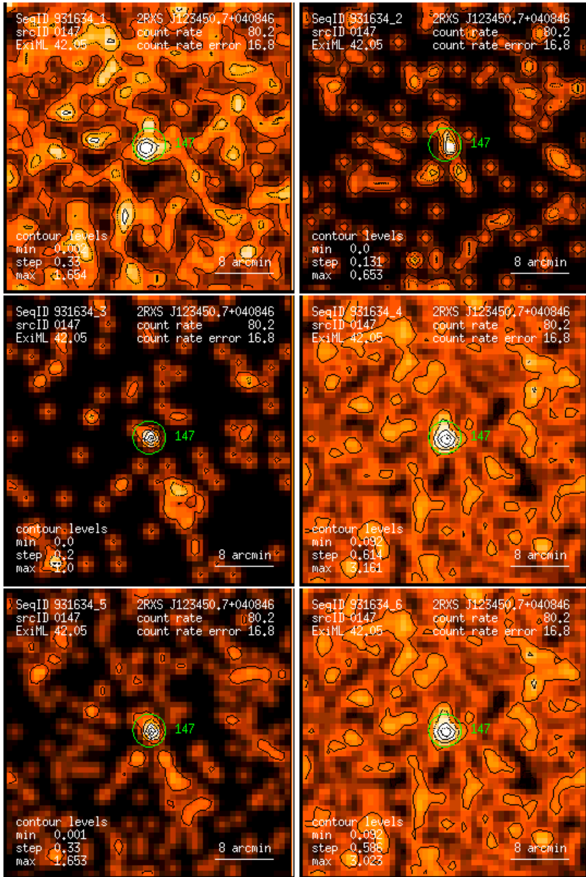
Figure 147: RASS 931634: detection 0147: band rate images, Gaussian filter: (1) PSPC channels 11 – 41, (2) 52 – 90, (3) 91 – 201, (4) 11 – 235, (5) 52 – 201, (6) 11 – 201. Broad band rates in counts/ks. Band rate contour levels in counts/ks/arcmin 2 .
