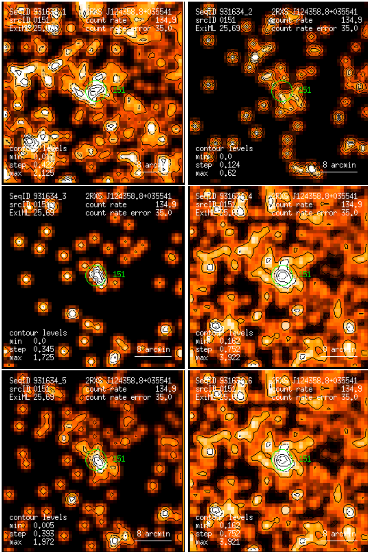
Figure 151: RASS 931634: detection 0151: band rate images, Gaussian filter: (1) PSPC channels 11 – 41, (2) 52 – 90, (3) 91 – 201, (4) 11 – 235, (5) 52 – 201, (6) 11 – 201. Broad band rates in counts/ks. Band rate contour levels in counts/ks/arcmin 2 .
