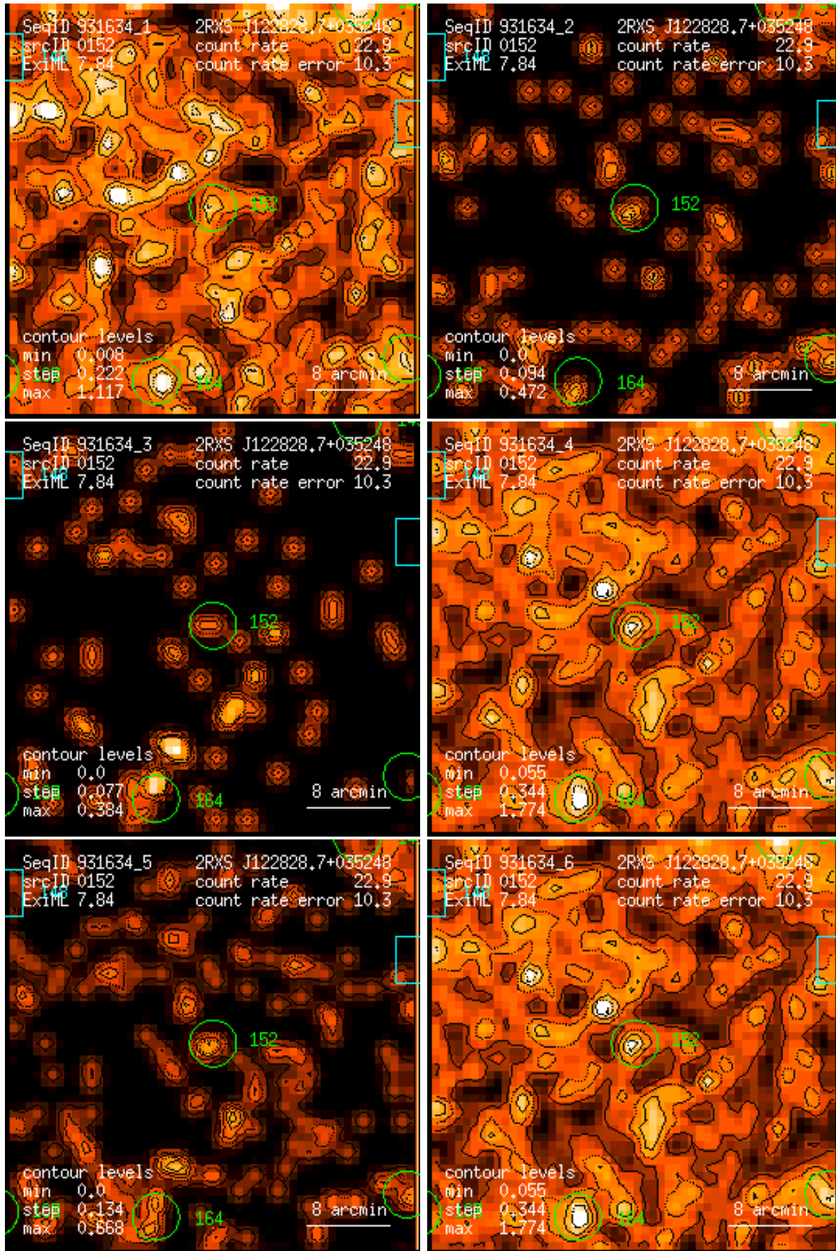
Figure 152: RASS 931634: detection 0152: band rate images, Gaussian filter: (1) PSPC channels 11 – 41, (2) 52 – 90, (3) 91 – 201, (4) 11 – 235, (5) 52 – 201, (6) 11 – 201. Broad band rates in counts/ks. Band rate contour levels in counts/ks/arcmin 2 .
