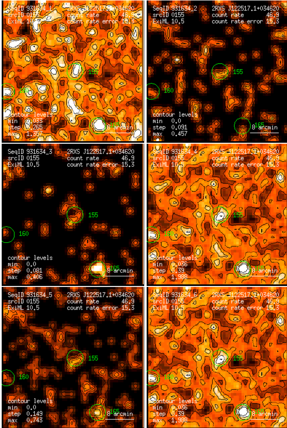
Figure 155: RASS 931634: detection 0155: band rate images, Gaussian filter: (1) PSPC channels 11 – 41, (2) 52 – 90, (3) 91 – 201, (4) 11 – 235, (5) 52 – 201, (6) 11 – 201. Broad band rates in counts/ks. Band rate contour levels in counts/ks/arcmin 2 .
