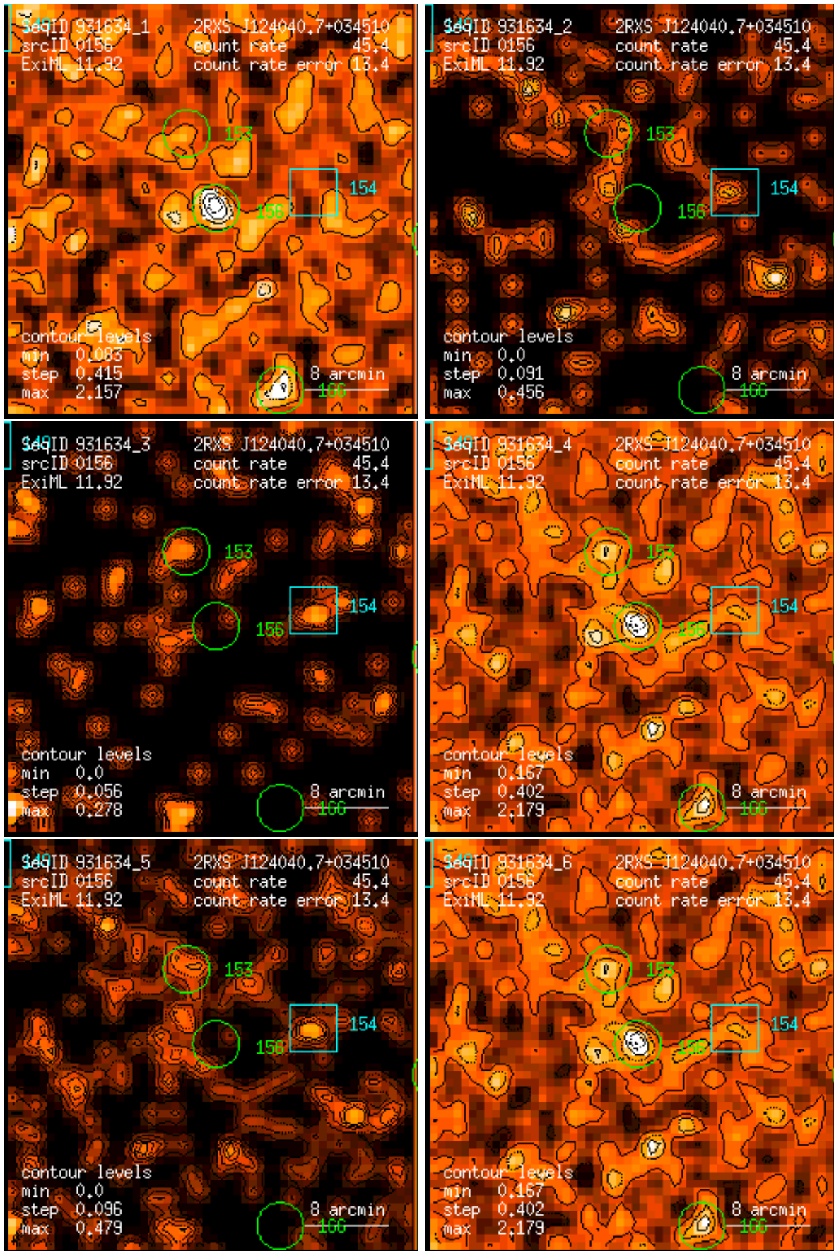
Figure 156: RASS 931634: detection 0156: band rate images, Gaussian filter: (1) PSPC channels 11 – 41, (2) 52 – 90, (3) 91 – 201, (4) 11 – 235, (5) 52 – 201, (6) 11 – 201. Broad band rates in counts/ks. Band rate contour levels in counts/ks/arcmin 2 .
