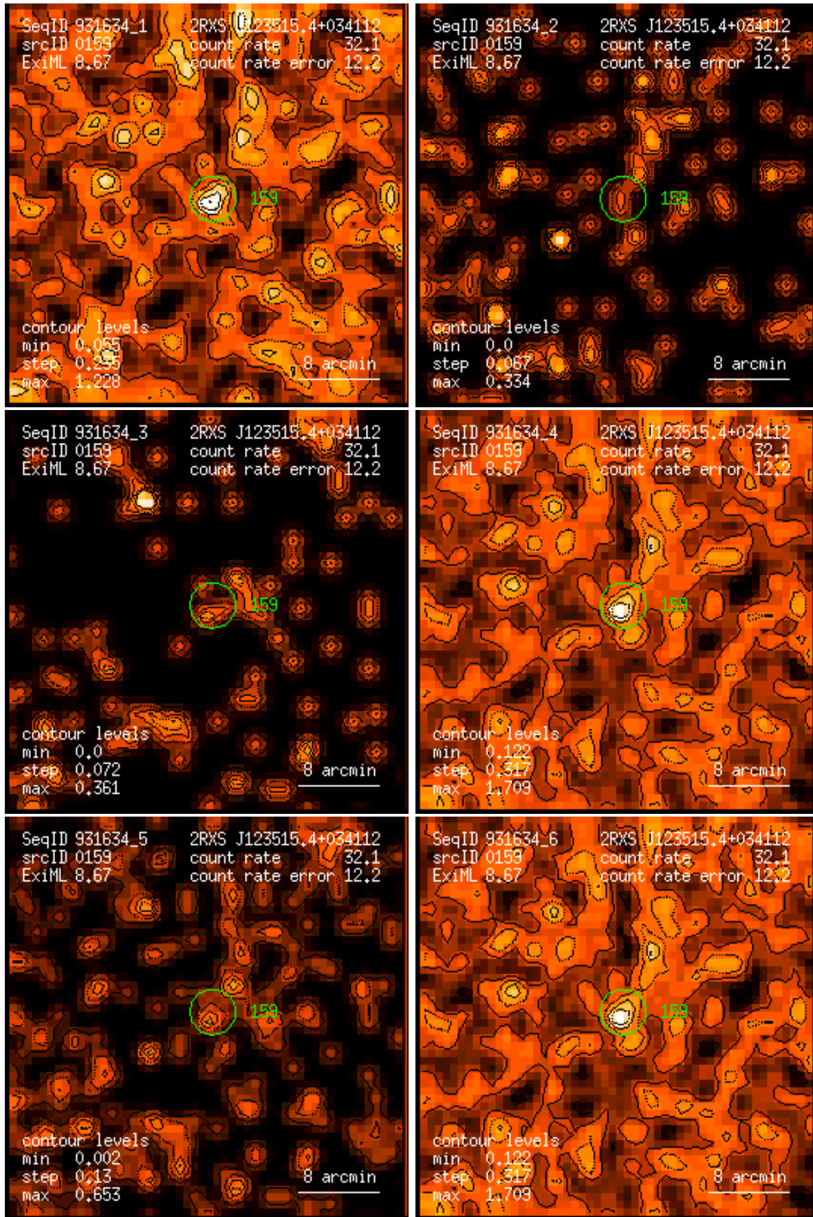
Figure 159: RASS 931634: detection 0159: band rate images, Gaussian filter: (1) PSPC channels 11 – 41, (2) 52 – 90, (3) 91 – 201, (4) 11 – 235, (5) 52 – 201, (6) 11 – 201. Broad band rates in counts/ks. Band rate contour levels in counts/ks/arcmin 2 .
