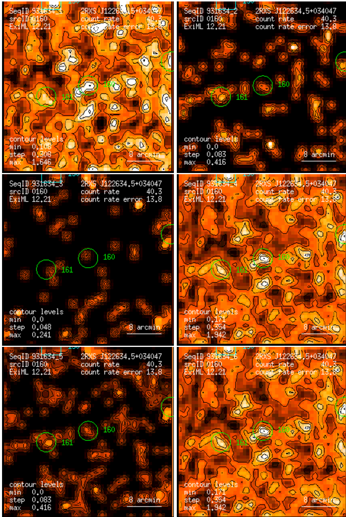
Figure 160: RASS 931634: detection 0160: band rate images, Gaussian filter: (1) PSPC channels 11 – 41, (2) 52 – 90, (3) 91 – 201, (4) 11 – 235, (5) 52 – 201, (6) 11 – 201. Broad band rates in counts/ks. Band rate contour levels in counts/ks/arcmin 2 .
