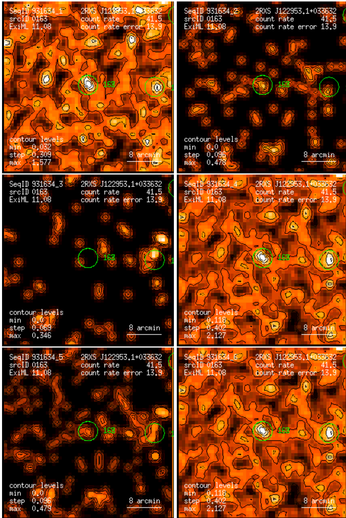
Figure 163: RASS 931634: detection 0163: band rate images, Gaussian filter: (1) PSPC channels 11 – 41, (2) 52 – 90, (3) 91 – 201, (4) 11 – 235, (5) 52 – 201, (6) 11 – 201. Broad band rates in counts/ks. Band rate contour levels in counts/ks/arcmin 2 .
