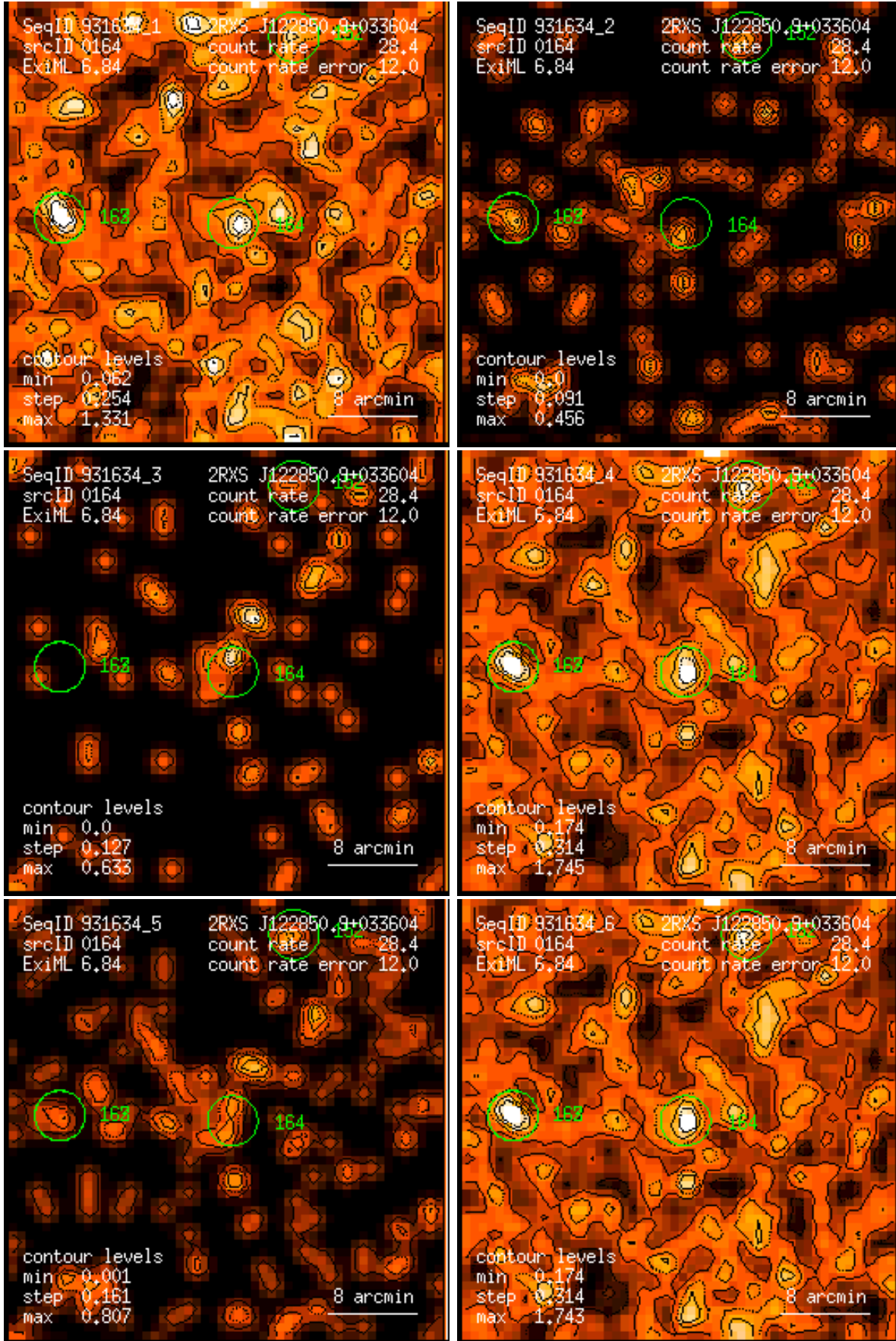
Figure 164: RASS 931634: detection 0164: band rate images, Gaussian filter: (1) PSPC channels 11 – 41, (2) 52 – 90, (3) 91 – 201, (4) 11 – 235, (5) 52 – 201, (6) 11 – 201. Broad band rates in counts/ks. Band rate contour levels in counts/ks/arcmin 2 .
