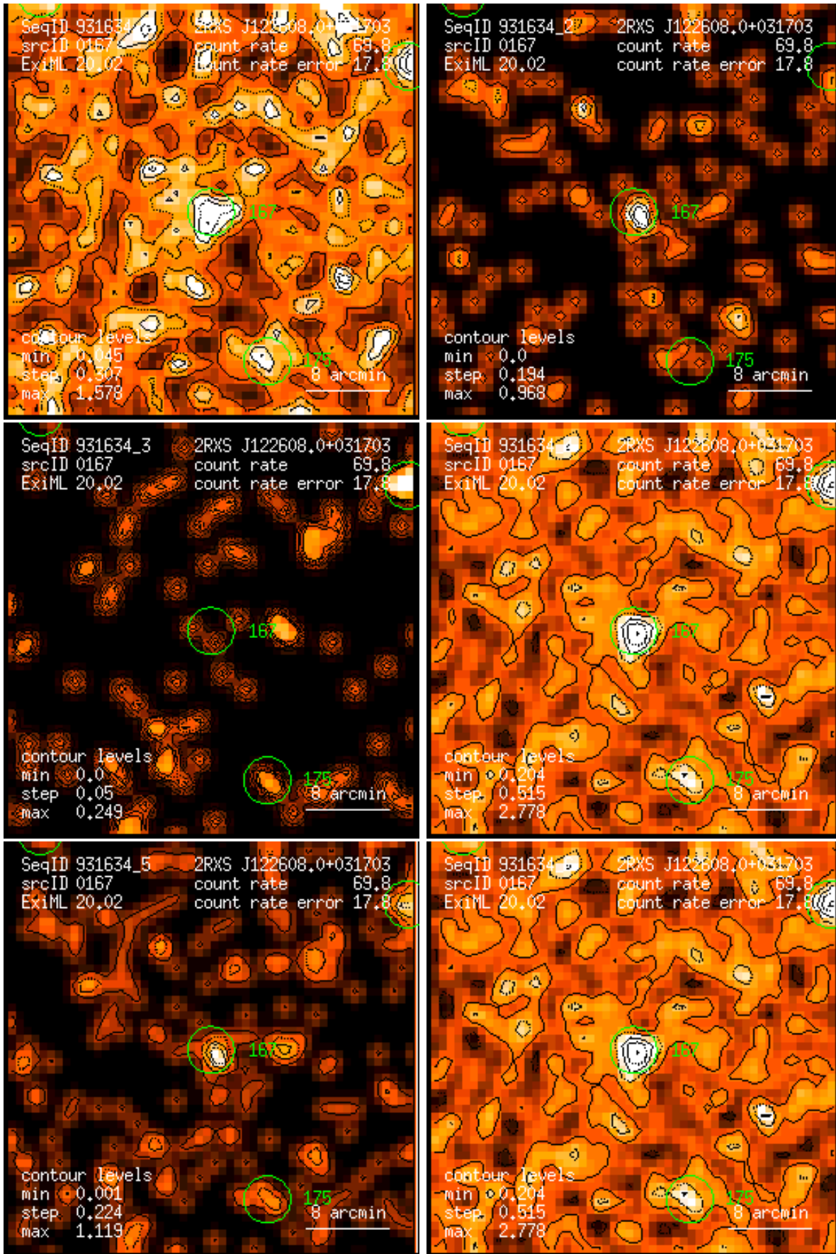
Figure 167: RASS 931634: detection 0167: band rate images, Gaussian filter: (1) PSPC channels 11 – 41, (2) 52 – 90, (3) 91 – 201, (4) 11 – 235, (5) 52 – 201, (6) 11 – 201. Broad band rates in counts/ks. Band rate contour levels in counts/ks/arcmin 2 .
