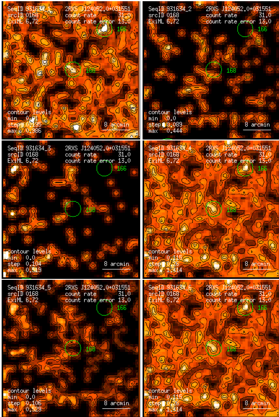
Figure 168: RASS 931634: detection 0168: band rate images, Gaussian filter: (1) PSPC channels 11 – 41, (2) 52 – 90, (3) 91 – 201, (4) 11 – 235, (5) 52 – 201, (6) 11 – 201. Broad band rates in counts/ks. Band rate contour levels in counts/ks/arcmin 2 .
