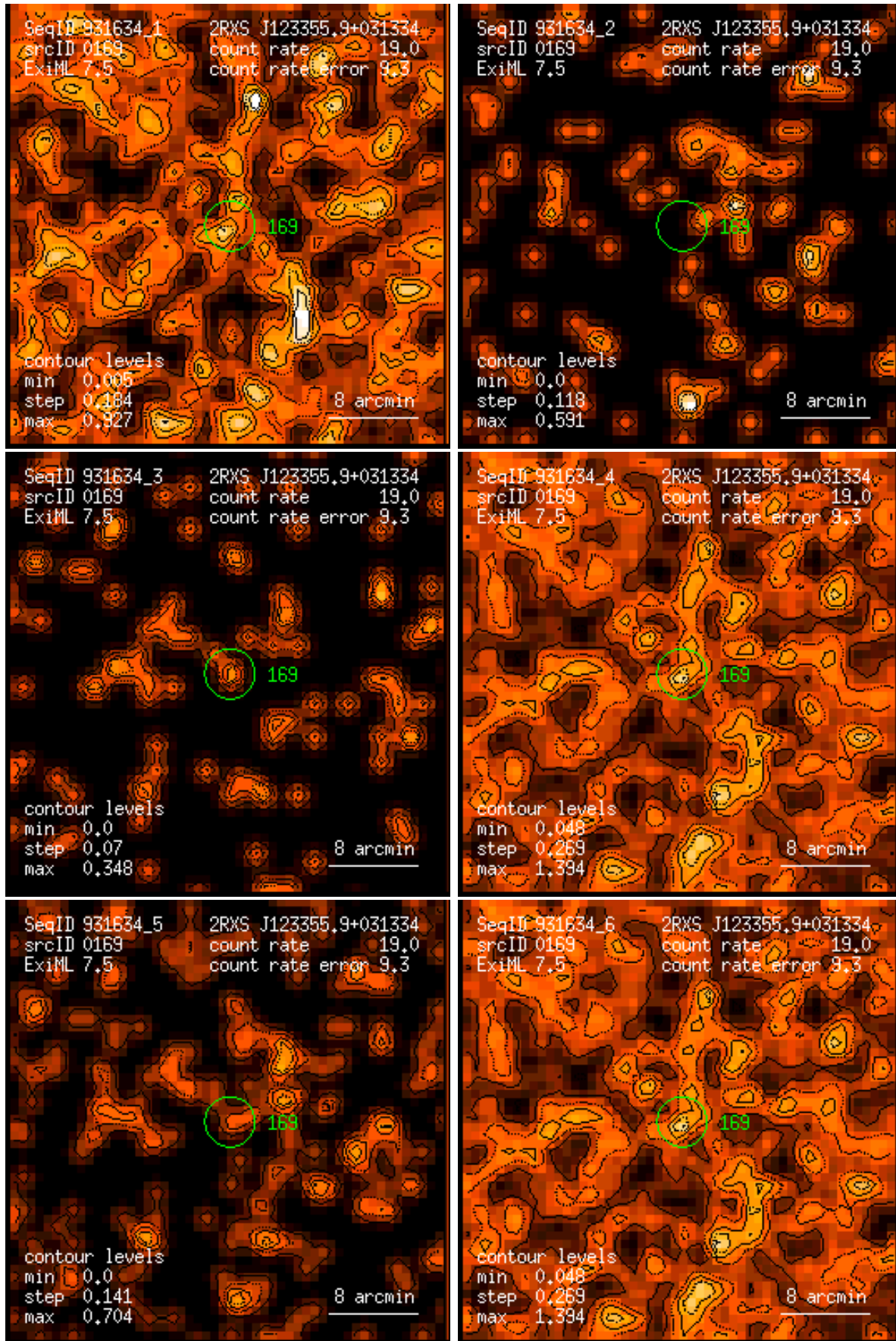
Figure 169: RASS 931634: detection 0169: band rate images, Gaussian filter: (1) PSPC channels 11 – 41, (2) 52 – 90, (3) 91 – 201, (4) 11 – 235, (5) 52 – 201, (6) 11 – 201. Broad band rates in counts/ks. Band rate contour levels in counts/ks/arcmin 2 .
