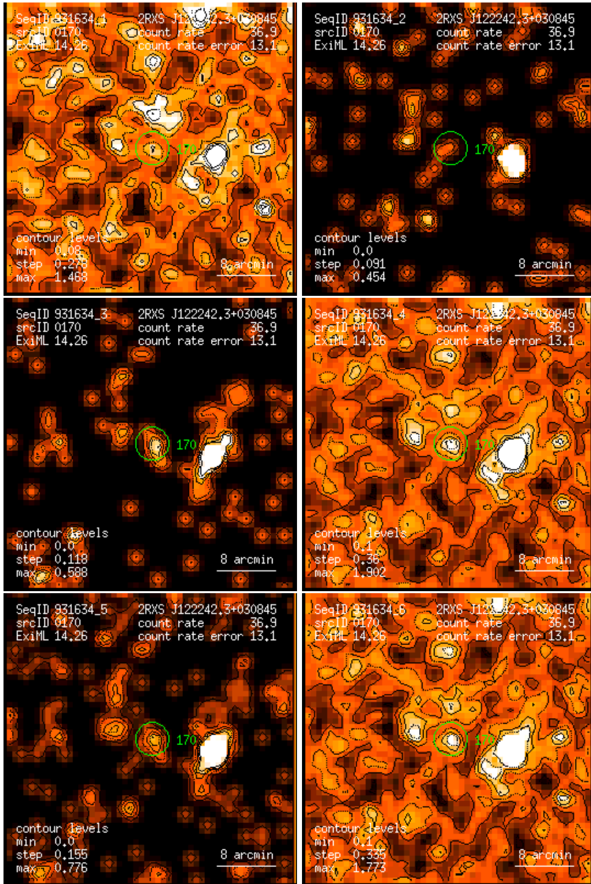
Figure 170: RASS 931634: detection 0170: band rate images, Gaussian filter: (1) PSPC channels 11 – 41, (2) 52 – 90, (3) 91 – 201, (4) 11 – 235, (5) 52 – 201, (6) 11 – 201. Broad band rates in counts/ks. Band rate contour levels in counts/ks/arcmin 2 .
